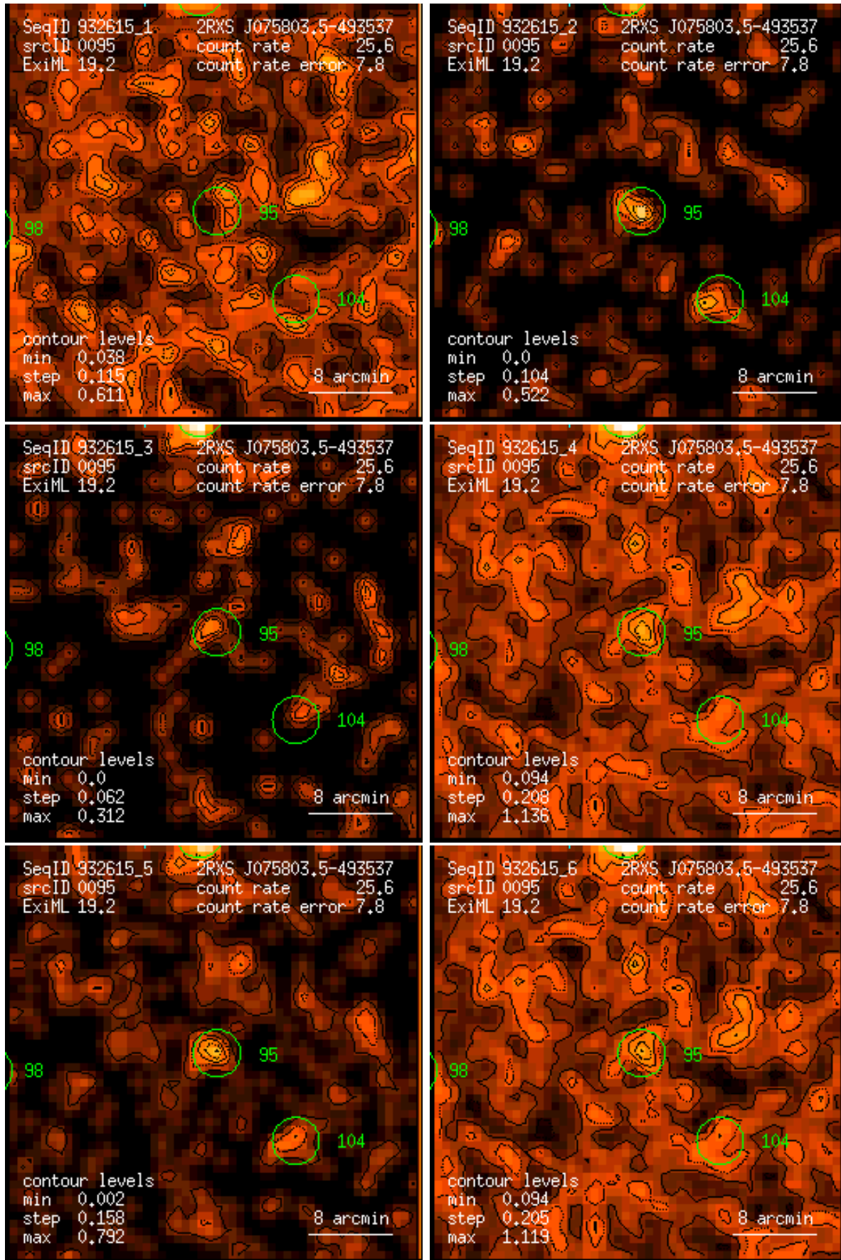
Figure 95: RASS 932615: detection 0095: band rate images, Gaussian filter: (1) PSPC channels 11 – 41, (2) 52 – 90, (3) 91 – 201, (4) 11 – 235, (5) 52 – 201, (6) 11 – 201. Broad band rates in counts/ks. Band rate contour levels in counts/ks/arcmin 2 .
