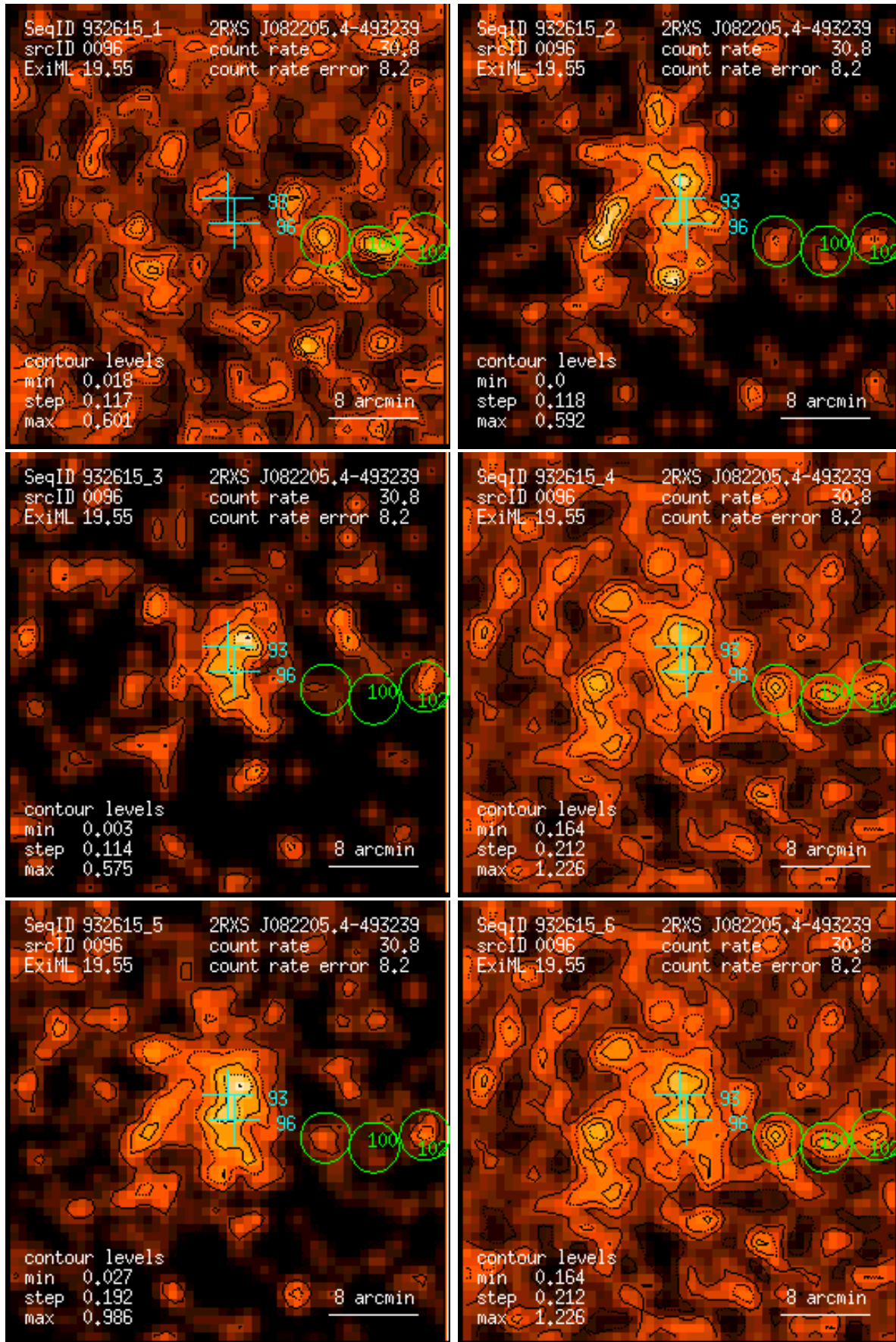
Figure 96: RASS 932615: detection 0096: band rate images, Gaussian filter: (1) PSPC channels 11 – 41, (2) 52 – 90, (3) 91 – 201, (4) 11 – 235, (5) 52 – 201, (6) 11 – 201. Broad band rates in counts/ks. Band rate contour levels in counts/ks/arcmin 2 .
