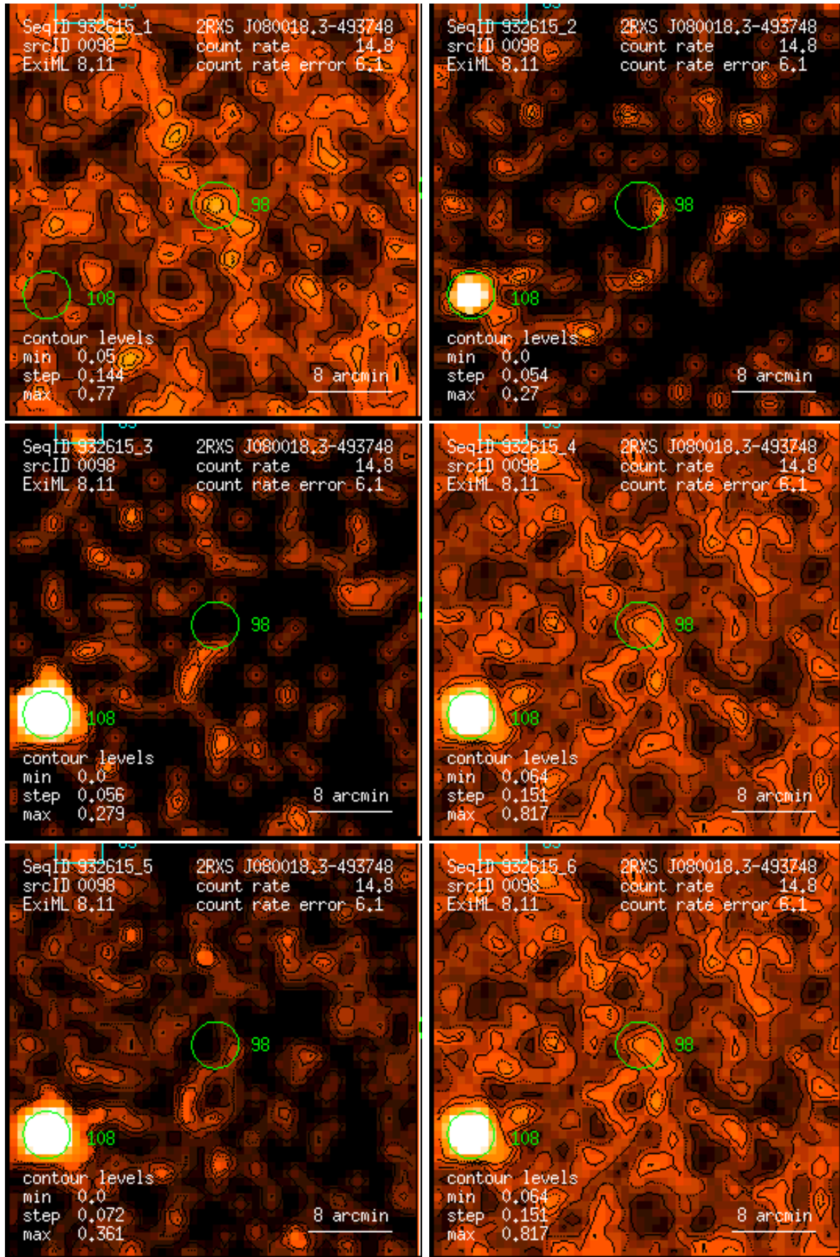
Figure 98: RASS 932615: detection 0098: band rate images, Gaussian filter: (1) PSPC channels 11 – 41, (2) 52 – 90, (3) 91 – 201, (4) 11 – 235, (5) 52 – 201, (6) 11 – 201. Broad band rates in counts/ks. Band rate contour levels in counts/ks/arcmin 2 .
