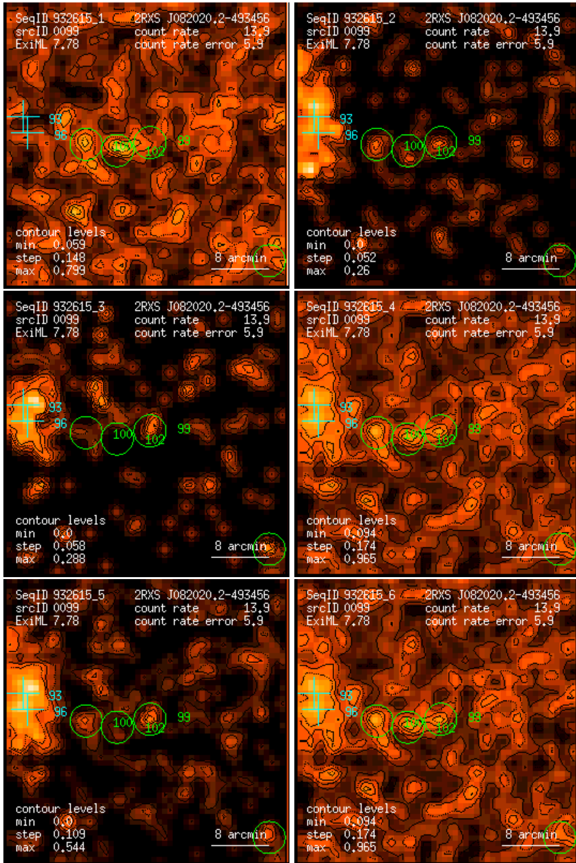
Figure 99: RASS 932615: detection 0099: band rate images, Gaussian filter: (1) PSPC channels 11 – 41, (2) 52 – 90, (3) 91 – 201, (4) 11 – 235, (5) 52 – 201, (6) 11 – 201. Broad band rates in counts/ks. Band rate contour levels in counts/ks/arcmin 2 .
