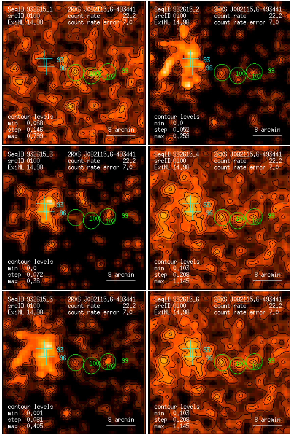
Figure 100: RASS 932615: detection 0100: band rate images, Gaussian filter: (1) PSPC channels 11 – 41, (2) 52 – 90, (3) 91 – 201, (4) 11 – 235, (5) 52 – 201, (6) 11 – 201. Broad band rates in counts/ks. Band rate contour levels in counts/ks/arcmin 2 .
