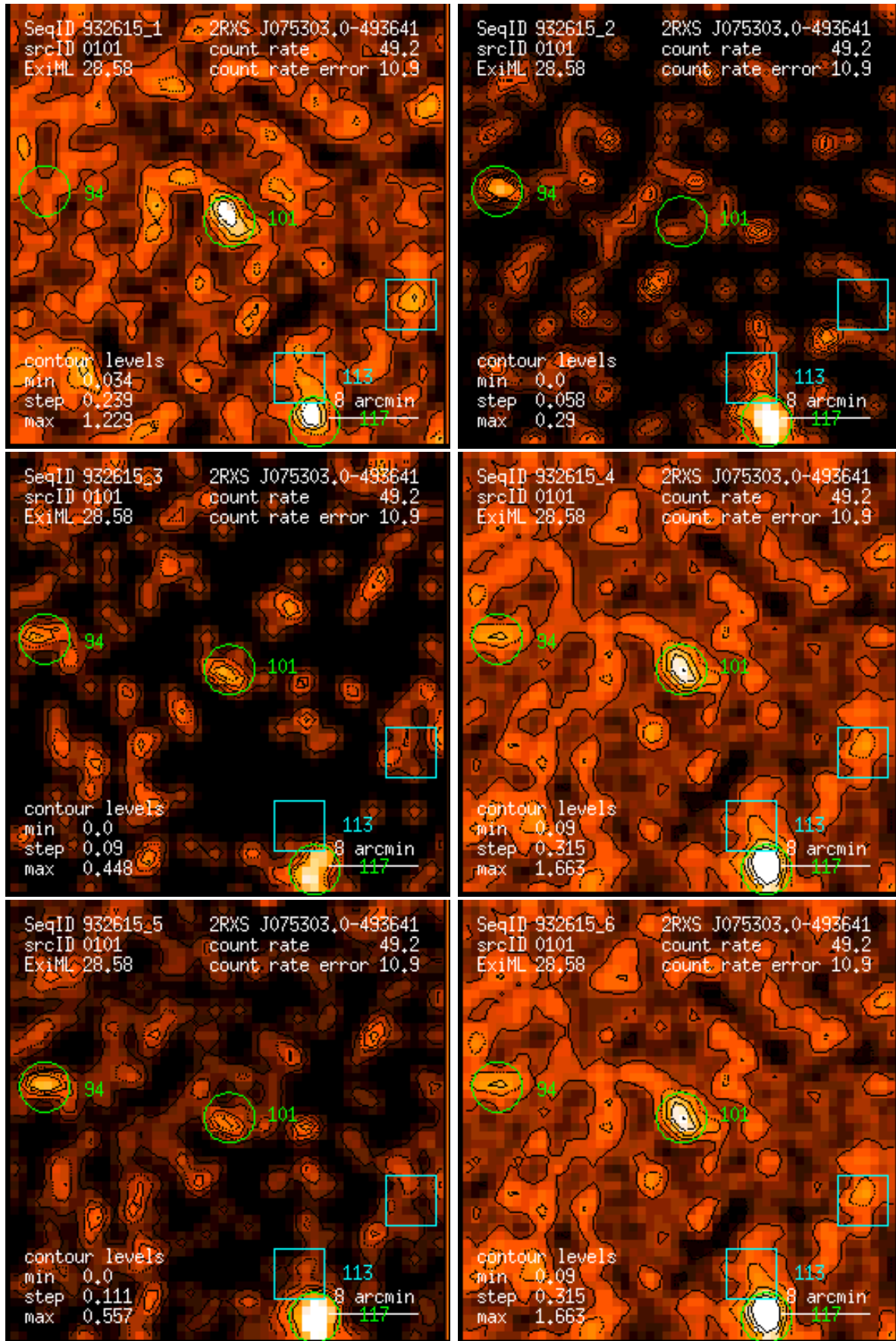
Figure 101: RASS 932615: detection 0101: band rate images, Gaussian filter: (1) PSPC channels 11 – 41, (2) 52 – 90, (3) 91 – 201, (4) 11 – 235, (5) 52 – 201, (6) 11 – 201. Broad band rates in counts/ks. Band rate contour levels in counts/ks/arcmin 2 .
