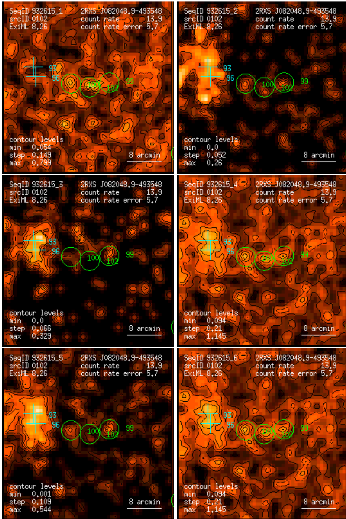
Figure 102: RASS 932615: detection 0102: band rate images, Gaussian filter: (1) PSPC channels 11 – 41, (2) 52 – 90, (3) 91 – 201, (4) 11 – 235, (5) 52 – 201, (6) 11 – 201. Broad band rates in counts/ks. Band rate contour levels in counts/ks/arcmin 2 .
