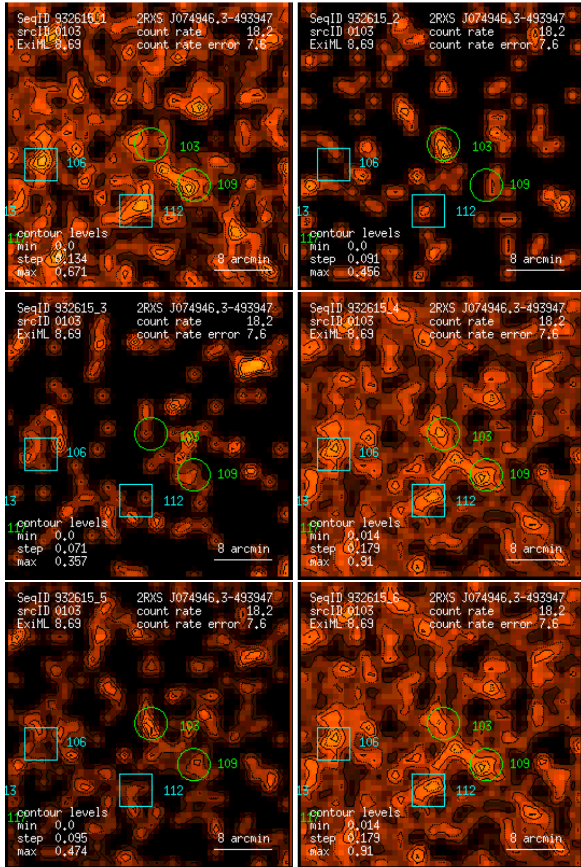
Figure 103: RASS 932615: detection 0103: band rate images, Gaussian filter: (1) PSPC channels 11 – 41, (2) 52 – 90, (3) 91 – 201, (4) 11 – 235, (5) 52 – 201, (6) 11 – 201. Broad band rates in counts/ks. Band rate contour levels in counts/ks/arcmin 2 .
