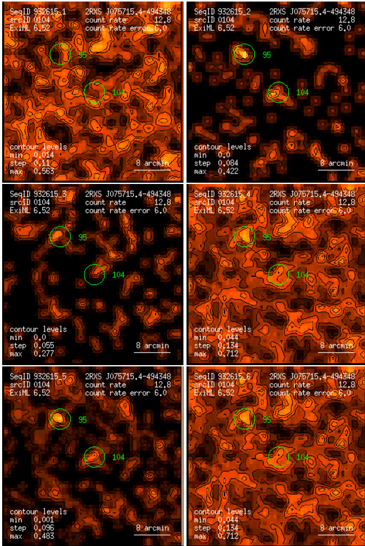
Figure 104: RASS 932615: detection 0104: band rate images, Gaussian filter: (1) PSPC channels 11 – 41, (2) 52 – 90, (3) 91 – 201, (4) 11 – 235, (5) 52 – 201, (6) 11 – 201. Broad band rates in counts/ks. Band rate contour levels in counts/ks/arcmin 2 .
