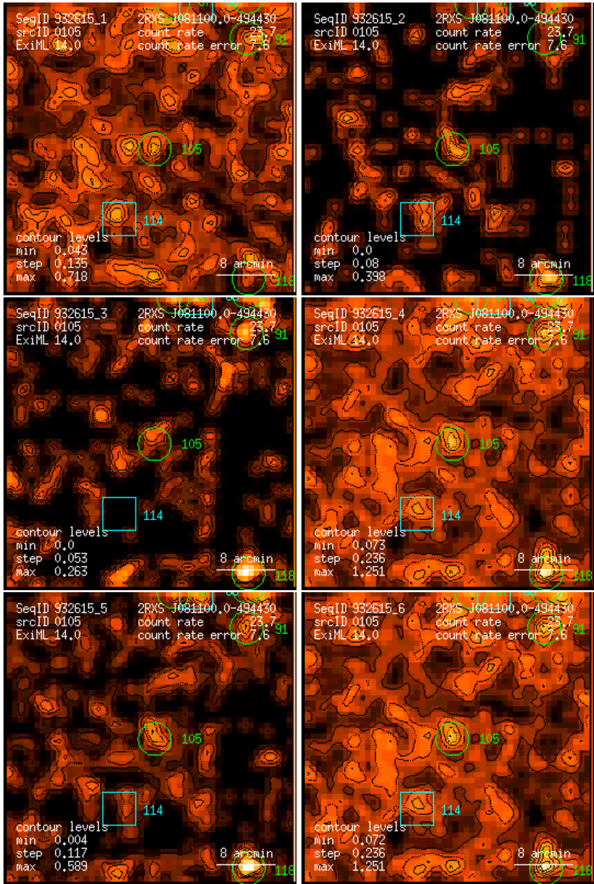
Figure 105: RASS 932615: detection 0105: band rate images, Gaussian filter: (1) PSPC channels 11 – 41, (2) 52 – 90, (3) 91 – 201, (4) 11 – 235, (5) 52 – 201, (6) 11 – 201. Broad band rates in counts/ks. Band rate contour levels in counts/ks/arcmin 2 .
