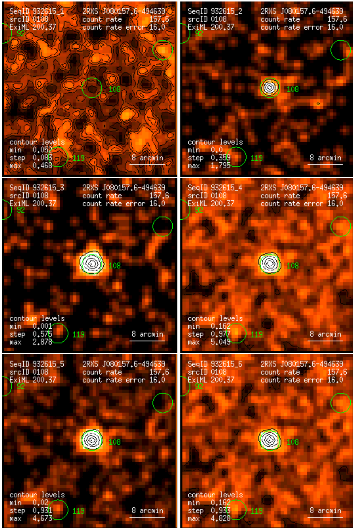
Figure 108: RASS 932615: detection 0108: band rate images, Gaussian filter: (1) PSPC channels 11 – 41, (2) 52 – 90, (3) 91 – 201, (4) 11 – 235, (5) 52 – 201, (6) 11 – 201. Broad band rates in counts/ks. Band rate contour levels in counts/ks/arcmin 2 .
