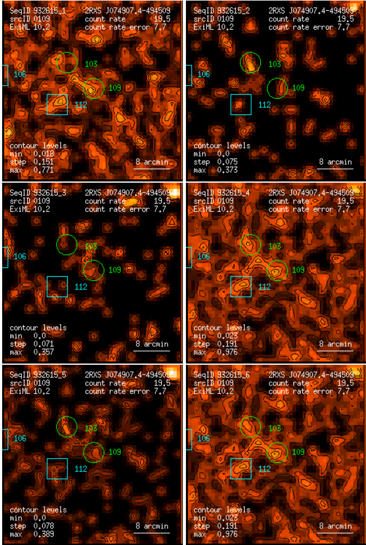
Figure 109: RASS 932615: detection 0109: band rate images, Gaussian filter: (1) PSPC channels 11 – 41, (2) 52 – 90, (3) 91 – 201, (4) 11 – 235, (5) 52 – 201, (6) 11 – 201. Broad band rates in counts/ks. Band rate contour levels in counts/ks/arcmin 2 .
