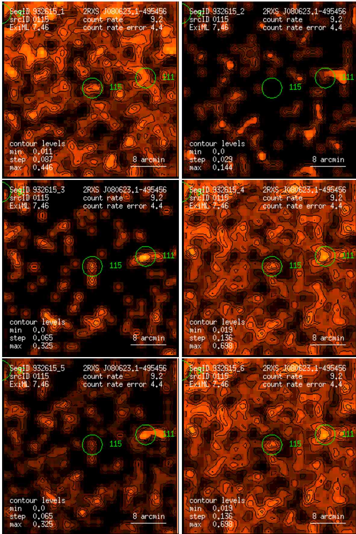
Figure 115: RASS 932615: detection 0115: band rate images, Gaussian filter: (1) PSPC channels 11 – 41, (2) 52 – 90, (3) 91 – 201, (4) 11 – 235, (5) 52 – 201, (6) 11 – 201. Broad band rates in counts/ks. Band rate contour levels in counts/ks/arcmin 2 .
