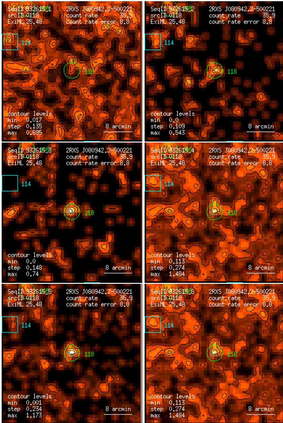
Figure 118: RASS 932615: detection 0118: band rate images, Gaussian filter: (1) PSPC channels 11 – 41, (2) 52 – 90, (3) 91 – 201, (4) 11 – 235, (5) 52 – 201, (6) 11 – 201. Broad band rates in counts/ks. Band rate contour levels in counts/ks/arcmin 2 .
