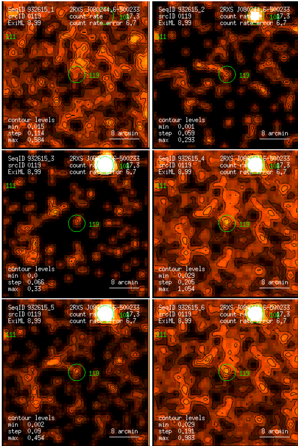
Figure 119: RASS 932615: detection 0119: band rate images, Gaussian filter: (1) PSPC channels 11 – 41, (2) 52 – 90, (3) 91 – 201, (4) 11 – 235, (5) 52 – 201, (6) 11 – 201. Broad band rates in counts/ks. Band rate contour levels in counts/ks/arcmin 2 .
