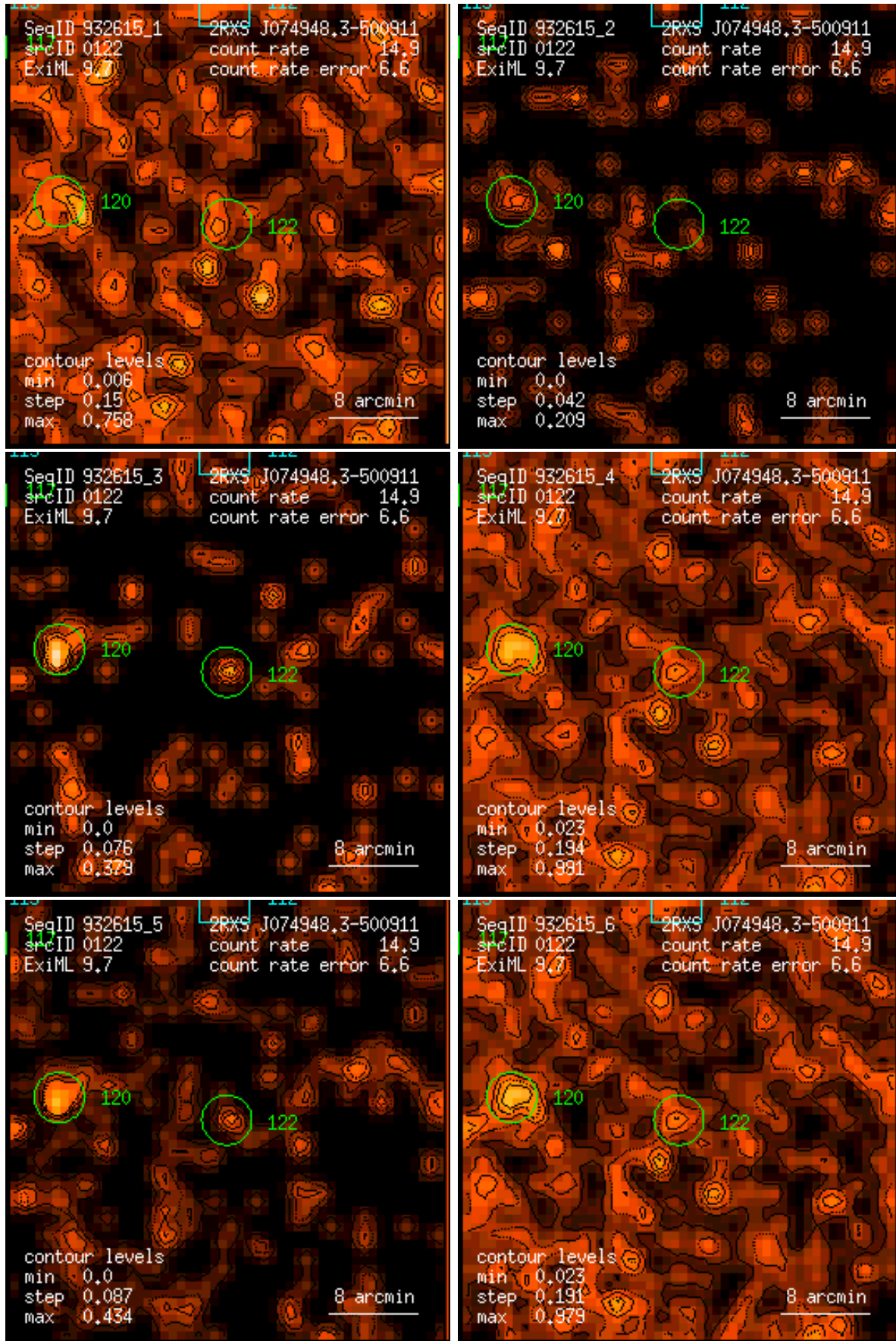
Figure 122: RASS 932615: detection 0122: band rate images, Gaussian filter: (1) PSPC channels 11 – 41, (2) 52 – 90, (3) 91 – 201, (4) 11 – 235, (5) 52 – 201, (6) 11 – 201. Broad band rates in counts/ks. Band rate contour levels in counts/ks/arcmin 2 .
