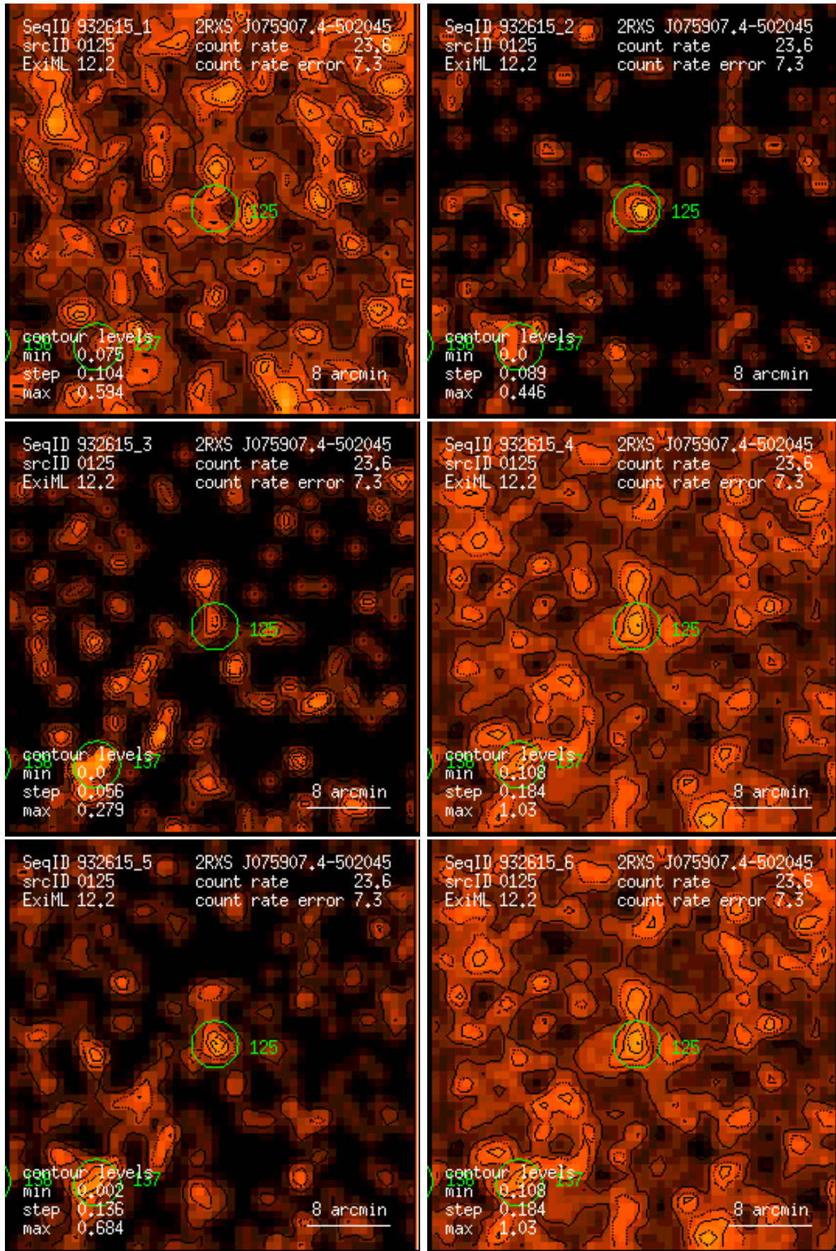
Figure 125: RASS 932615: detection 0125: band rate images, Gaussian filter: (1) PSPC channels 11 – 41, (2) 52 – 90, (3) 91 – 201, (4) 11 – 235, (5) 52 – 201, (6) 11 – 201. Broad band rates in counts/ks. Band rate contour levels in counts/ks/arcmin 2 .
