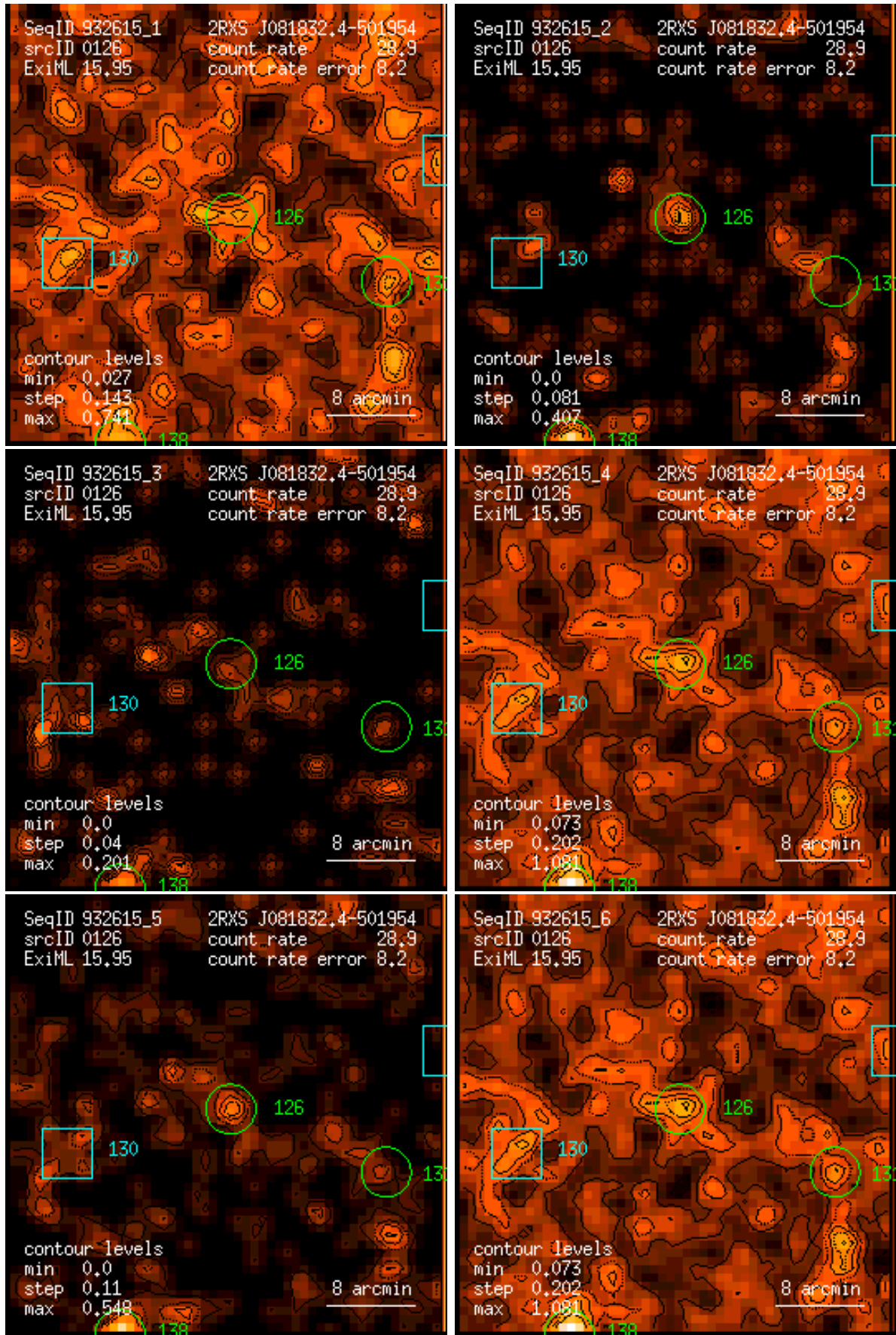
Figure 126: RASS 932615: detection 0126: band rate images, Gaussian filter: (1) PSPC channels 11 – 41, (2) 52 – 90, (3) 91 – 201, (4) 11 – 235, (5) 52 – 201, (6) 11 – 201. Broad band rates in counts/ks. Band rate contour levels in counts/ks/arcmin 2 .
