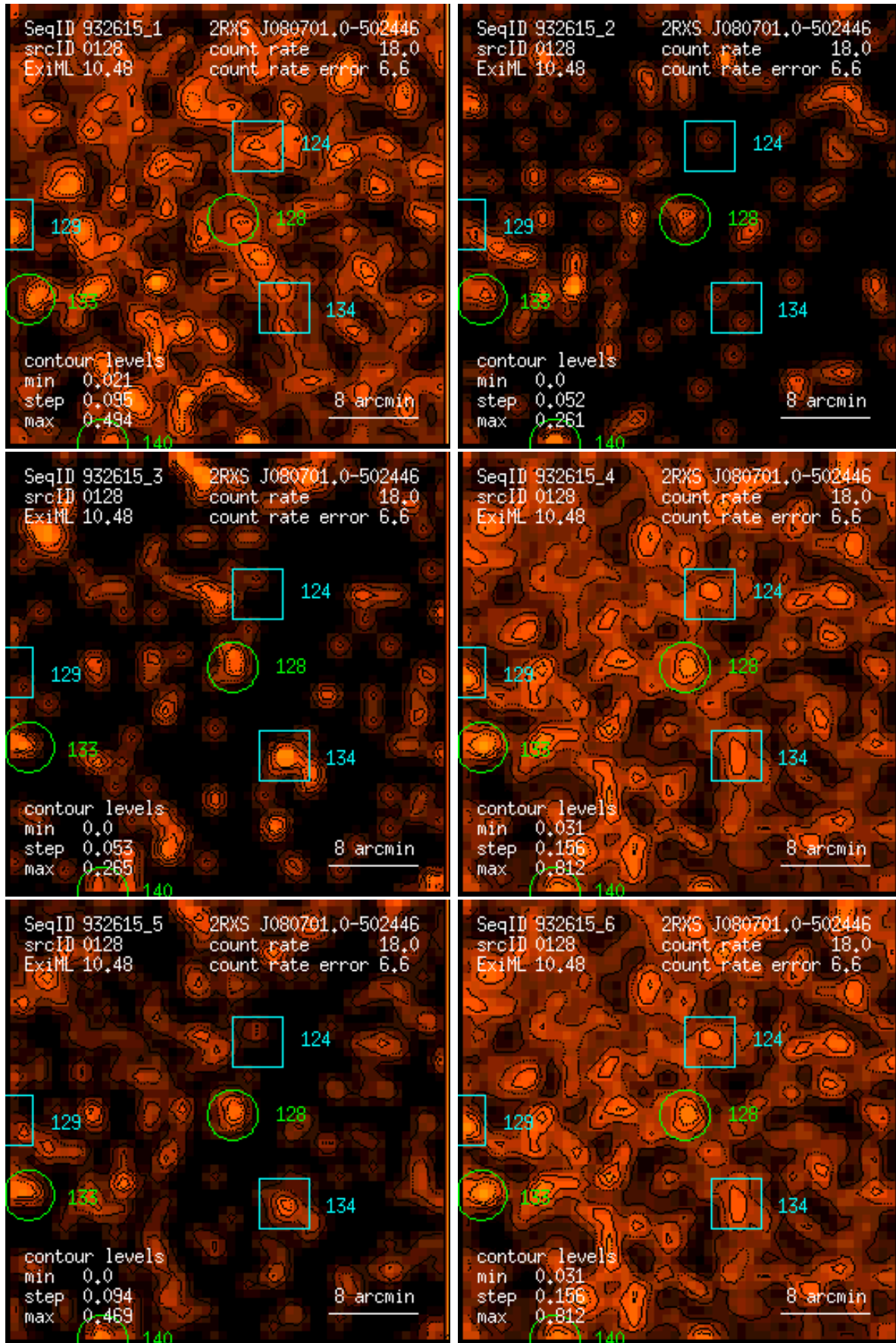
Figure 128: RASS 932615: detection 0128: band rate images, Gaussian filter: (1) PSPC channels 11 – 41, (2) 52 – 90, (3) 91 – 201, (4) 11 – 235, (5) 52 – 201, (6) 11 – 201. Broad band rates in counts/ks. Band rate contour levels in counts/ks/arcmin 2 .
