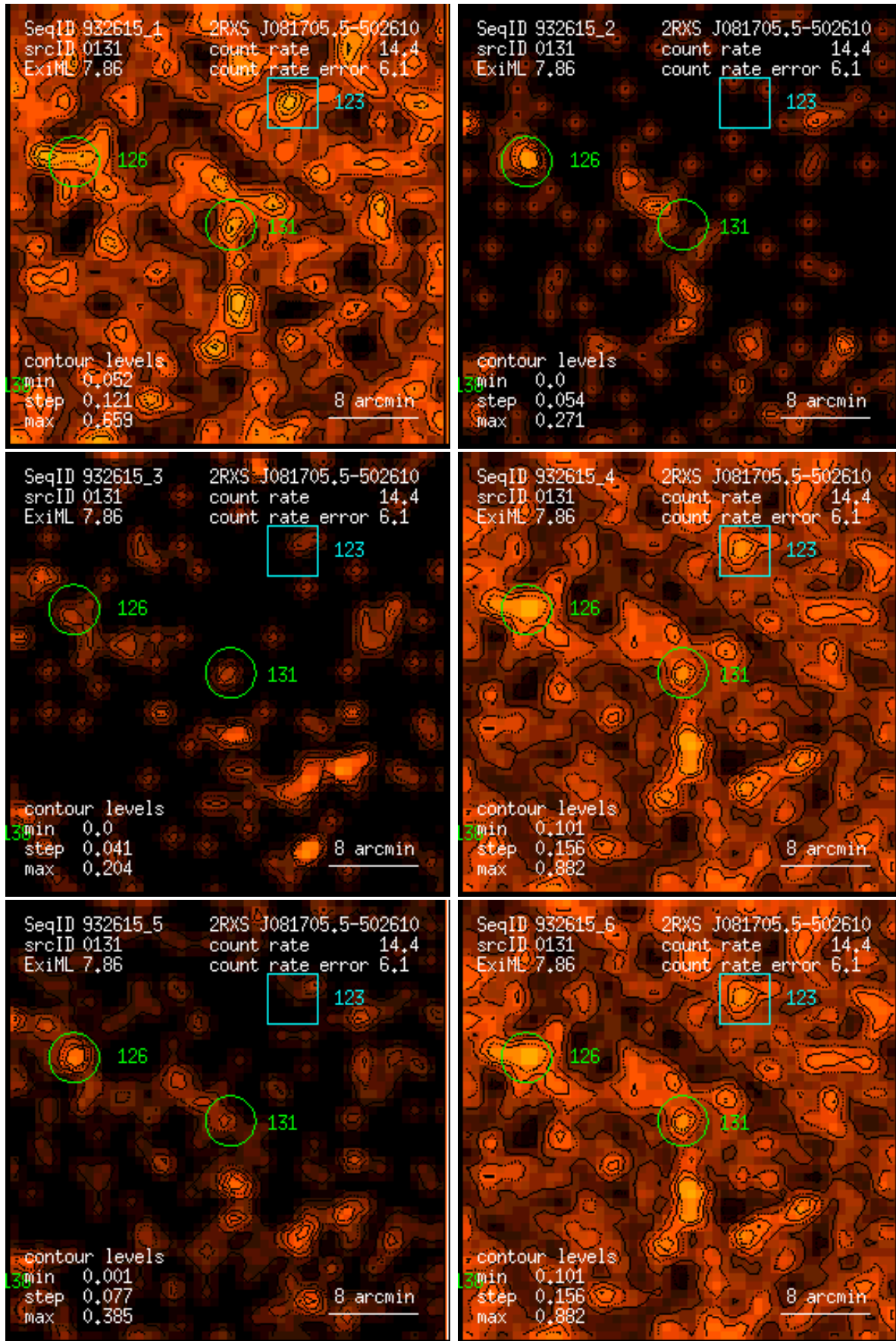
Figure 131: RASS 932615: detection 0131: band rate images, Gaussian filter: (1) PSPC channels 11 – 41, (2) 52 – 90, (3) 91 – 201, (4) 11 – 235, (5) 52 – 201, (6) 11 – 201. Broad band rates in counts/ks. Band rate contour levels in counts/ks/arcmin 2 .
