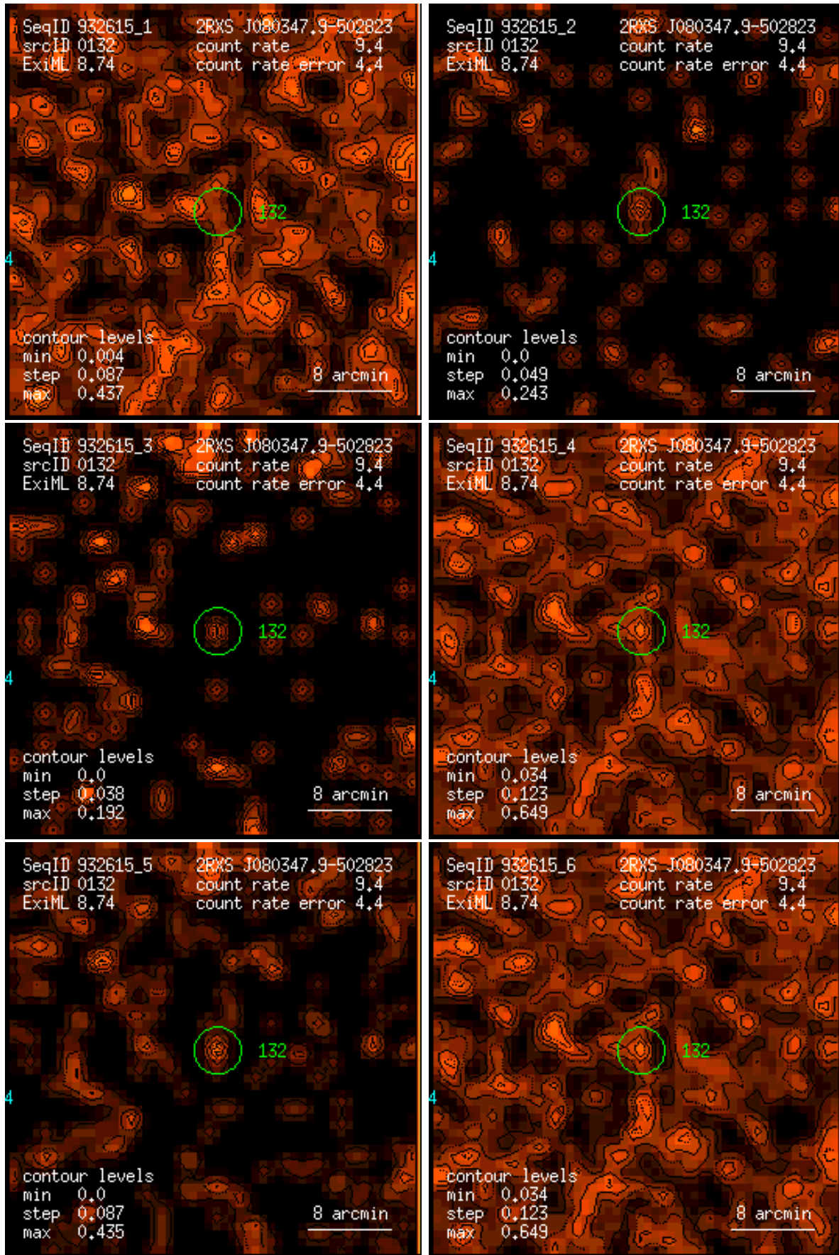
Figure 132: RASS 932615: detection 0132: band rate images, Gaussian filter: (1) PSPC channels 11 – 41, (2) 52 – 90, (3) 91 – 201, (4) 11 – 235, (5) 52 – 201, (6) 11 – 201. Broad band rates in counts/ks. Band rate contour levels in counts/ks/arcmin 2 .
