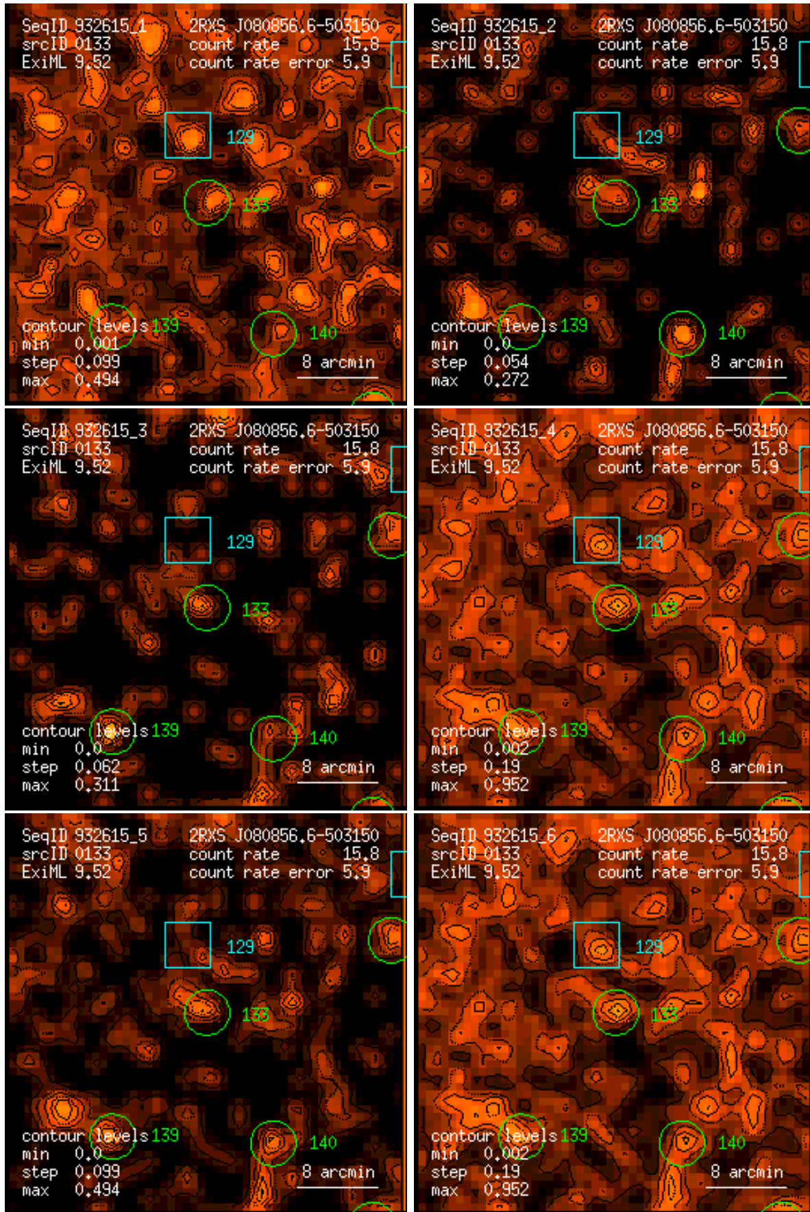
Figure 133: RASS 932615: detection 0133: band rate images, Gaussian filter: (1) PSPC channels 11 – 41, (2) 52 – 90, (3) 91 – 201, (4) 11 – 235, (5) 52 – 201, (6) 11 – 201. Broad band rates in counts/ks. Band rate contour levels in counts/ks/arcmin 2 .
