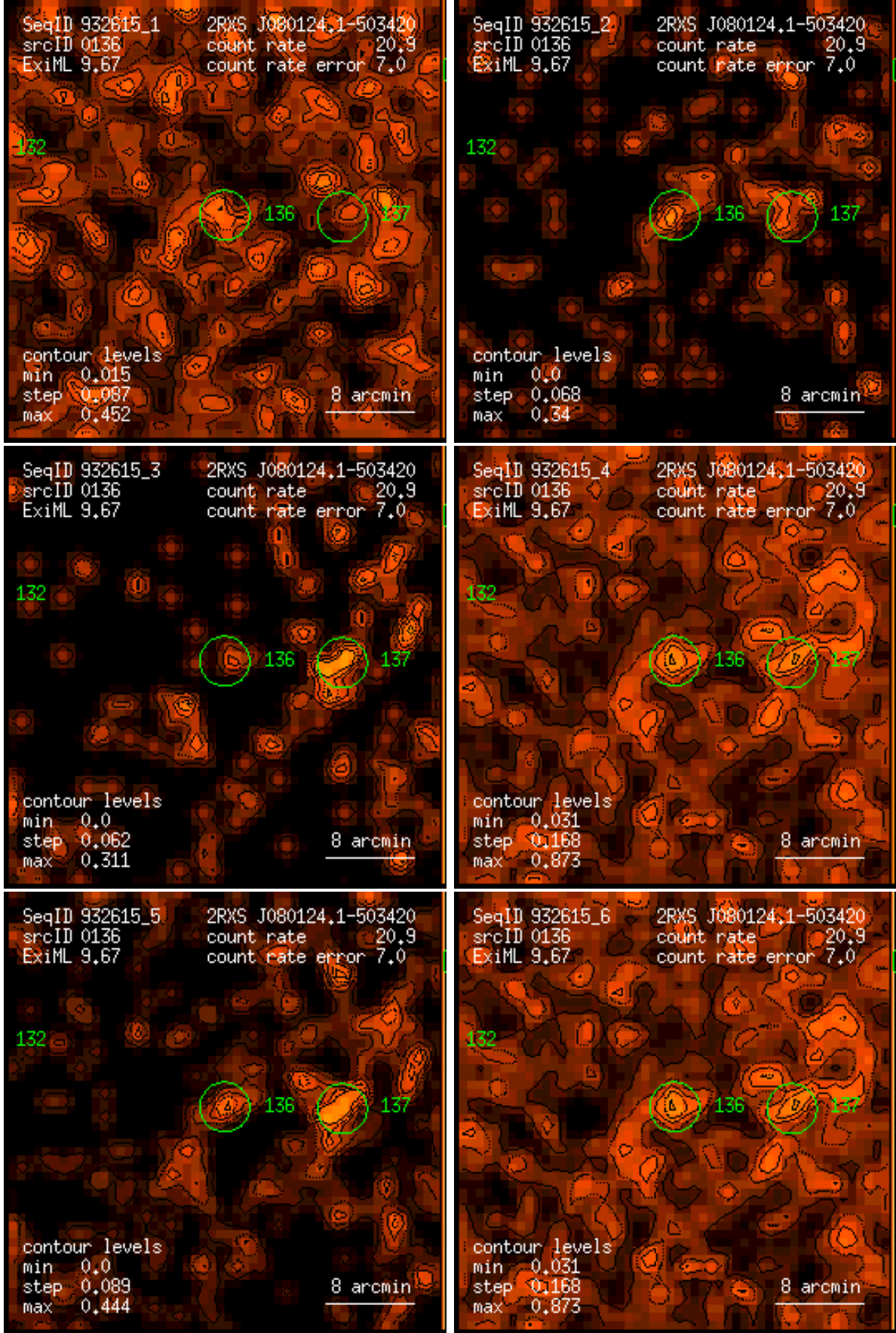
Figure 136: RASS 932615: detection 0136: band rate images, Gaussian filter: (1) PSPC channels 11 – 41, (2) 52 – 90, (3) 91 – 201, (4) 11 – 235, (5) 52 – 201, (6) 11 – 201. Broad band rates in counts/ks. Band rate contour levels in counts/ks/arcmin 2 .
