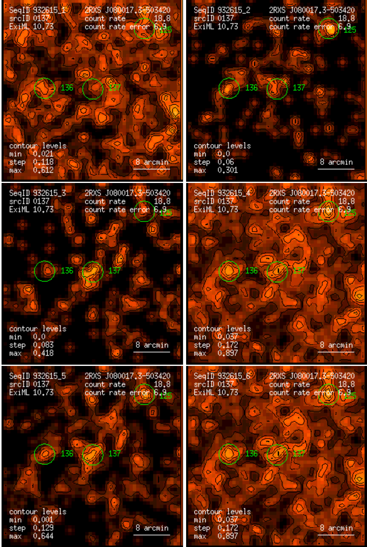
Figure 137: RASS 932615: detection 0137: band rate images, Gaussian filter: (1) PSPC channels 11 – 41, (2) 52 – 90, (3) 91 – 201, (4) 11 – 235, (5) 52 – 201, (6) 11 – 201. Broad band rates in counts/ks. Band rate contour levels in counts/ks/arcmin 2 .
