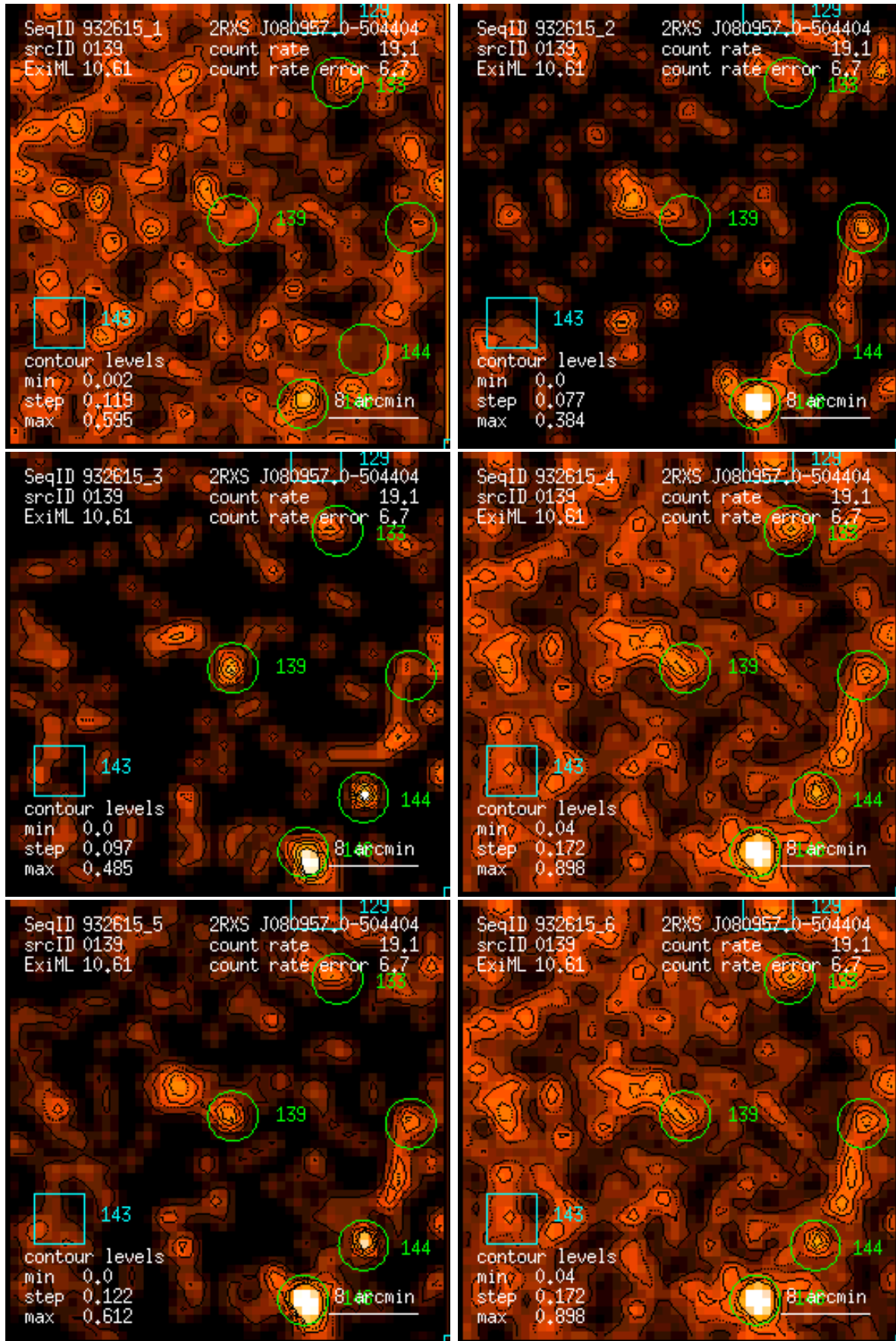
Figure 139: RASS 932615: detection 0139: band rate images, Gaussian filter: (1) PSPC channels 11 – 41, (2) 52 – 90, (3) 91 – 201, (4) 11 – 235, (5) 52 – 201, (6) 11 – 201. Broad band rates in counts/ks. Band rate contour levels in counts/ks/arcmin 2 .
