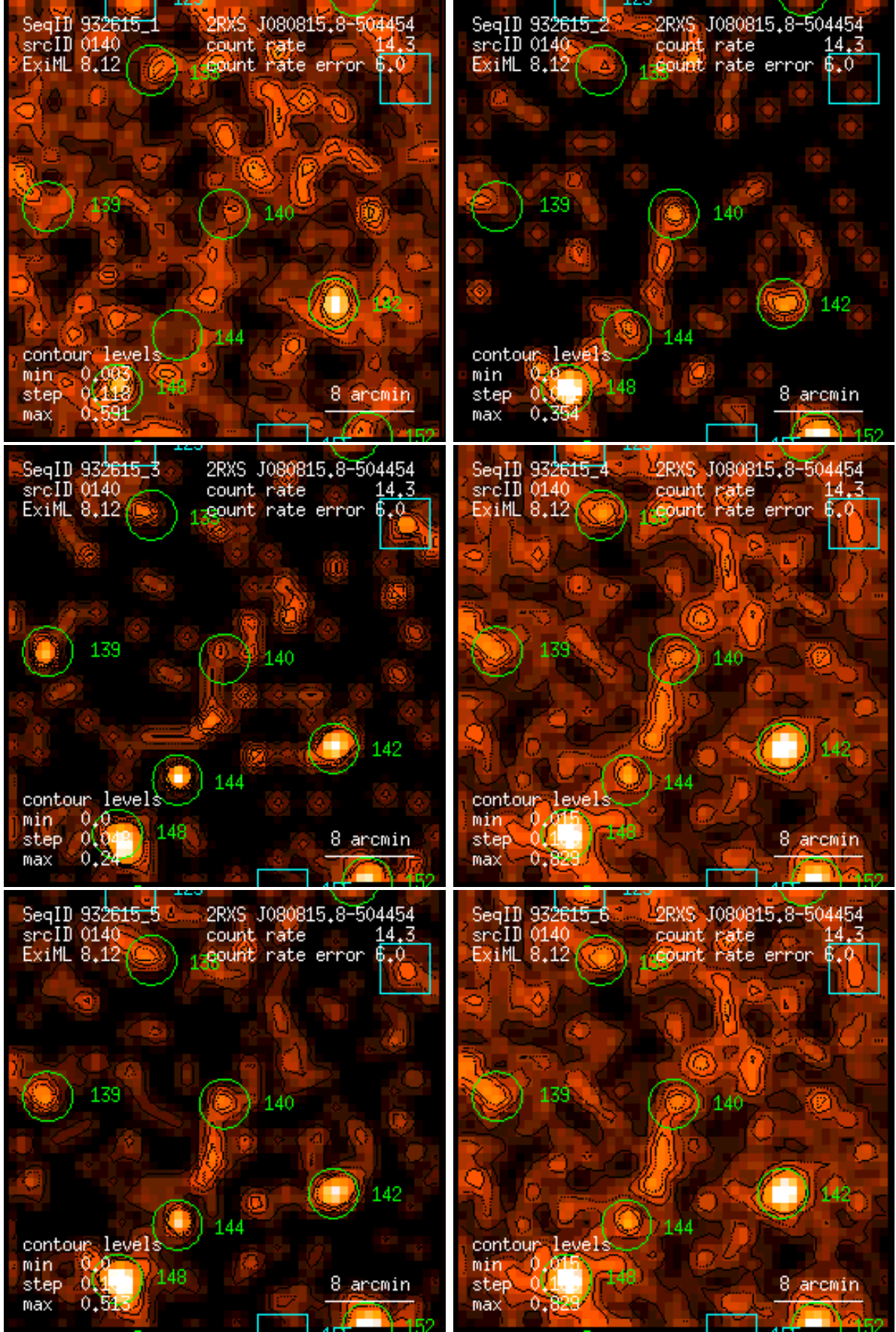
Figure 140: RASS 932615: detection 0140: band rate images, Gaussian filter: (1) PSPC channels 11 – 41, (2) 52 – 90, (3) 91 – 201, (4) 11 – 235, (5) 52 – 201, (6) 11 – 201. Broad band rates in counts/ks. Band rate contour levels in counts/ks/arcmin 2 .
