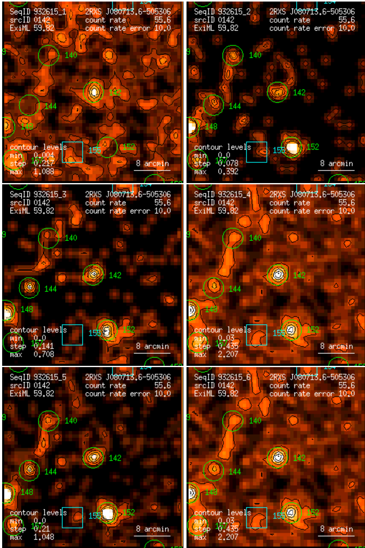
Figure 142: RASS 932615: detection 0142: band rate images, Gaussian filter: (1) PSPC channels 11 – 41, (2) 52 – 90, (3) 91 – 201, (4) 11 – 235, (5) 52 – 201, (6) 11 – 201. Broad band rates in counts/ks. Band rate contour levels in counts/ks/arcmin 2 .
