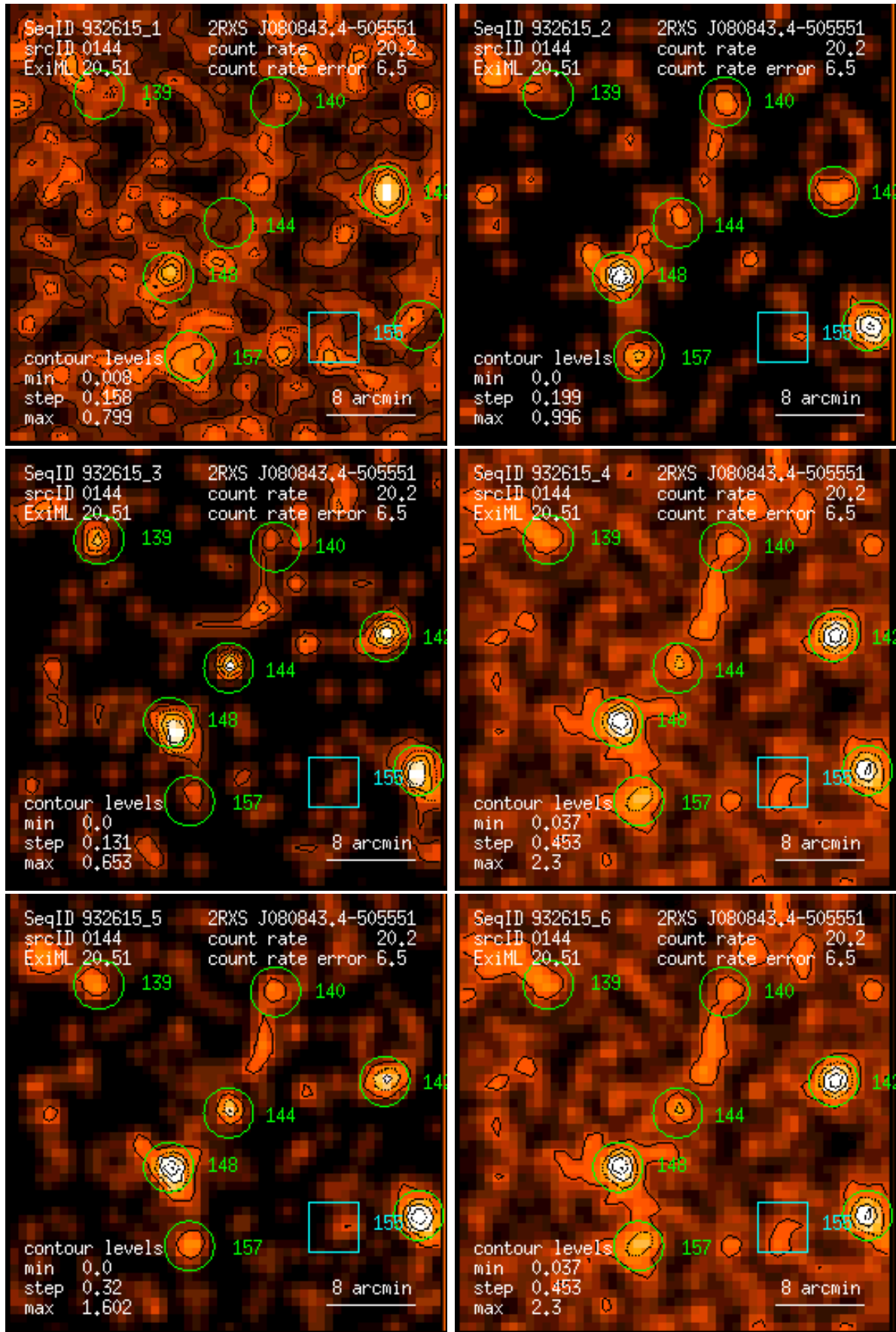
Figure 144: RASS 932615: detection 0144: band rate images, Gaussian filter: (1) PSPC channels 11 – 41, (2) 52 – 90, (3) 91 – 201, (4) 11 – 235, (5) 52 – 201, (6) 11 – 201. Broad band rates in counts/ks. Band rate contour levels in counts/ks/arcmin 2 .
