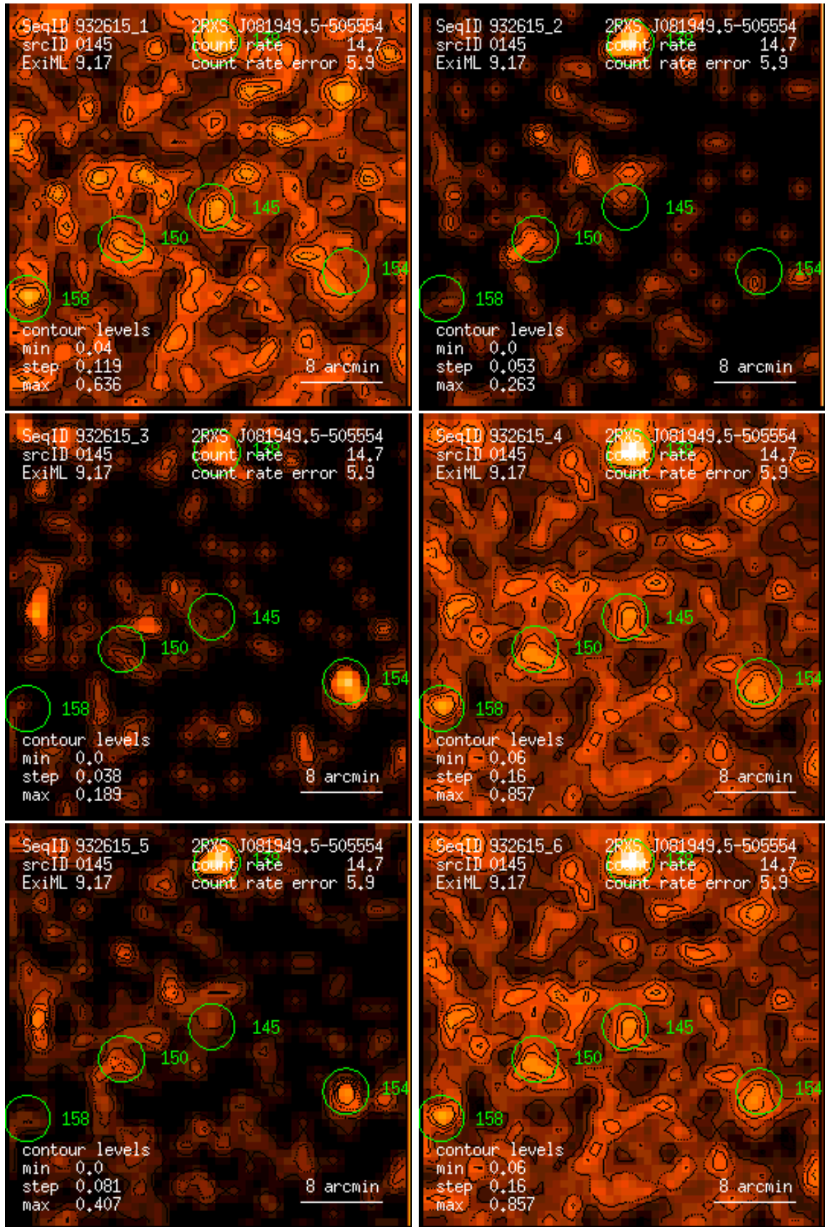
Figure 145: RASS 932615: detection 0145: band rate images, Gaussian filter: (1) PSPC channels 11 – 41, (2) 52 – 90, (3) 91 – 201, (4) 11 – 235, (5) 52 – 201, (6) 11 – 201. Broad band rates in counts/ks. Band rate contour levels in counts/ks/arcmin 2 .
