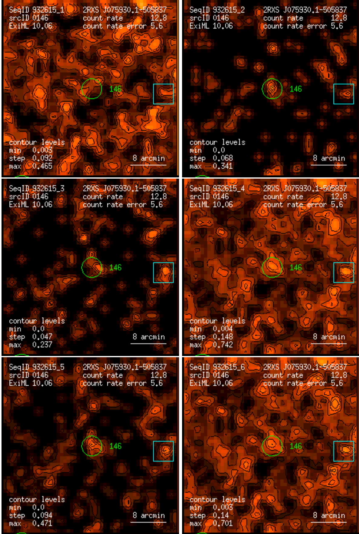
Figure 146: RASS 932615: detection 0146: band rate images, Gaussian filter: (1) PSPC channels 11 – 41, (2) 52 – 90, (3) 91 – 201, (4) 11 – 235, (5) 52 – 201, (6) 11 – 201. Broad band rates in counts/ks. Band rate contour levels in counts/ks/arcmin 2 .
