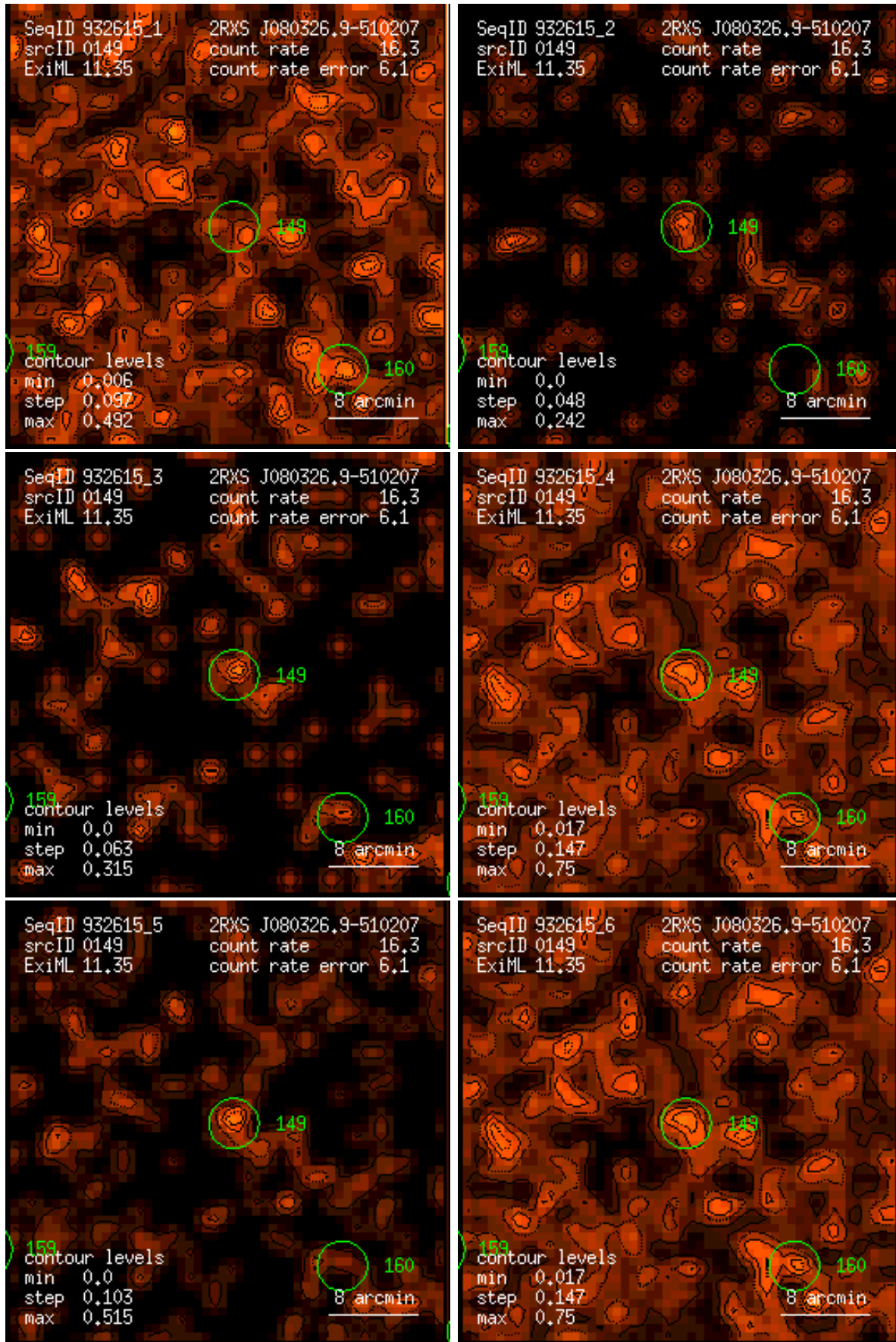
Figure 149: RASS 932615: detection 0149: band rate images, Gaussian filter: (1) PSPC channels 11 – 41, (2) 52 – 90, (3) 91 – 201, (4) 11 – 235, (5) 52 – 201, (6) 11 – 201. Broad band rates in counts/ks. Band rate contour levels in counts/ks/arcmin 2 .
