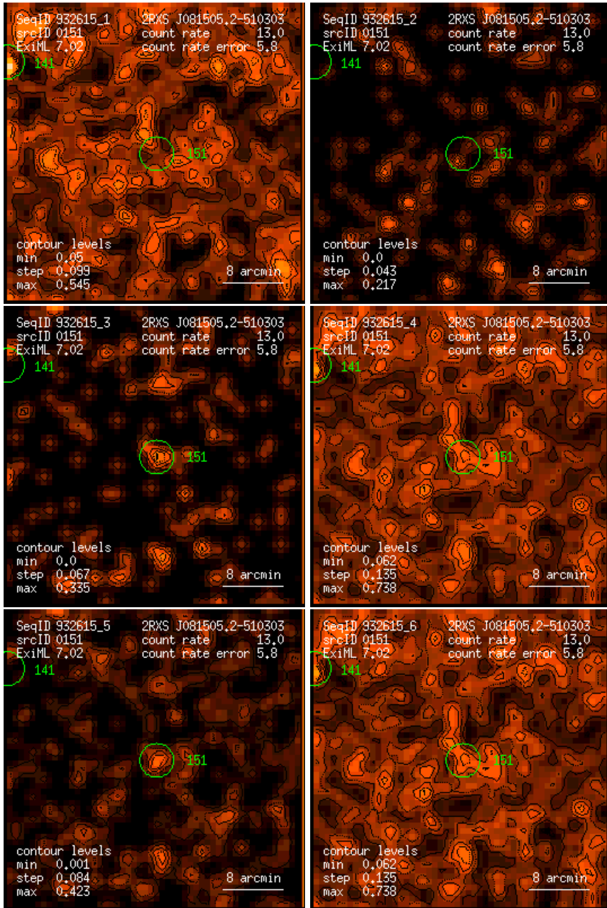
Figure 151: RASS 932615: detection 0151: band rate images, Gaussian filter: (1) PSPC channels 11 – 41, (2) 52 – 90, (3) 91 – 201, (4) 11 – 235, (5) 52 – 201, (6) 11 – 201. Broad band rates in counts/ks. Band rate contour levels in counts/ks/arcmin 2 .
