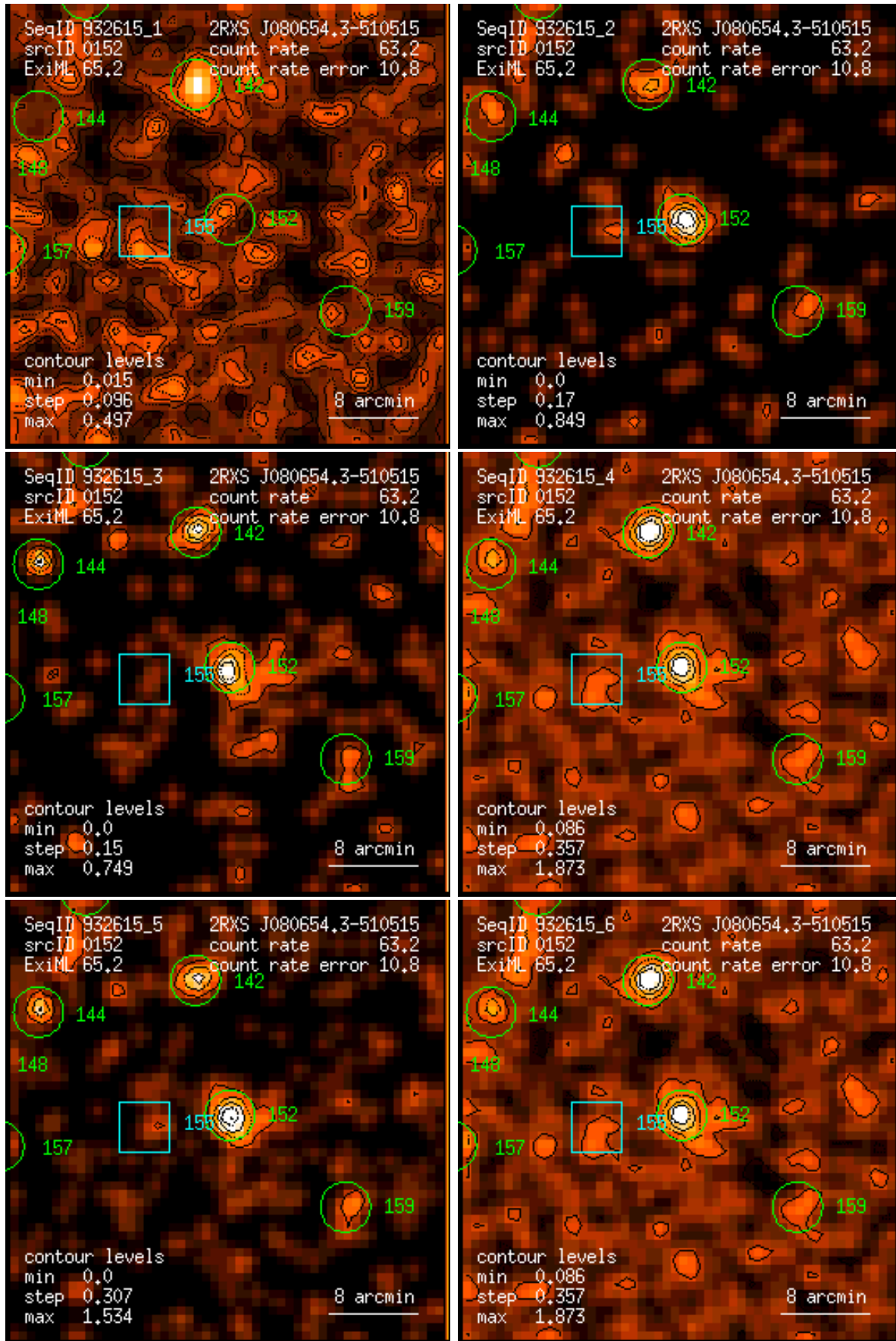
Figure 152: RASS 932615: detection 0152: band rate images, Gaussian filter: (1) PSPC channels 11 – 41, (2) 52 – 90, (3) 91 – 201, (4) 11 – 235, (5) 52 – 201, (6) 11 – 201. Broad band rates in counts/ks. Band rate contour levels in counts/ks/arcmin 2 .
