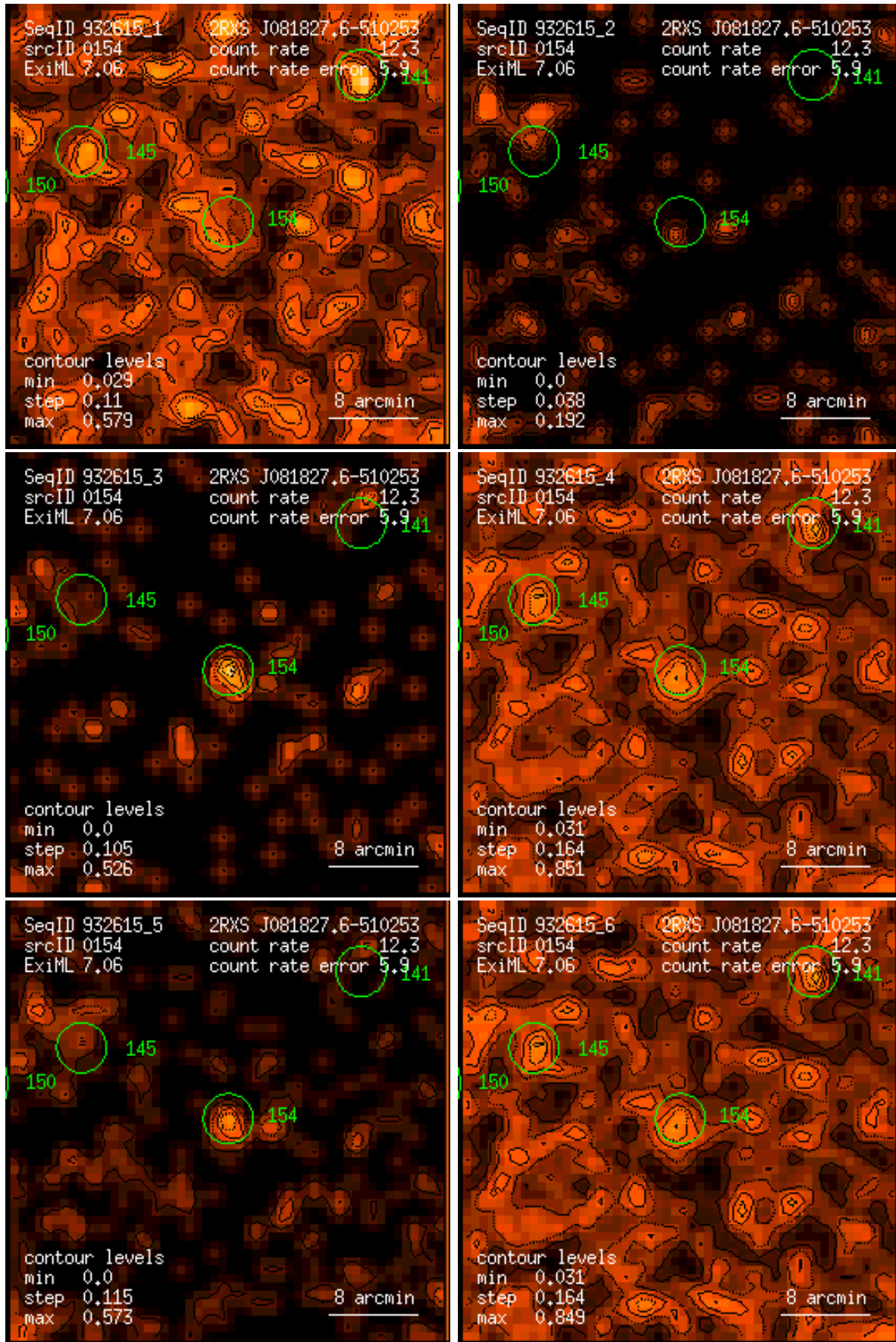
Figure 154: RASS 932615: detection 0154: band rate images, Gaussian filter: (1) PSPC channels 11 – 41, (2) 52 – 90, (3) 91 – 201, (4) 11 – 235, (5) 52 – 201, (6) 11 – 201. Broad band rates in counts/ks. Band rate contour levels in counts/ks/arcmin 2 .
