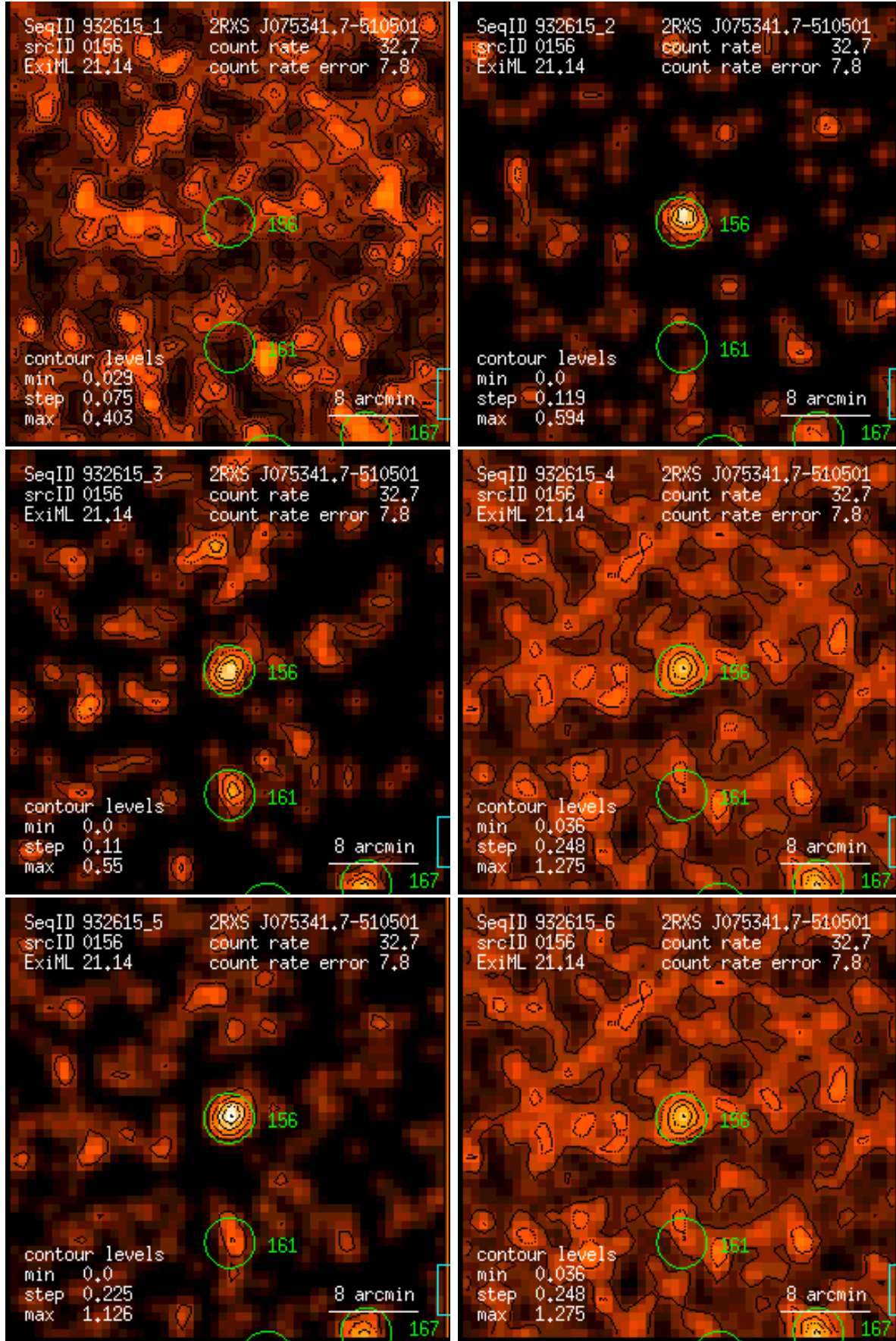
Figure 156: RASS 932615: detection 0156: band rate images, Gaussian filter: (1) PSPC channels 11 – 41, (2) 52 – 90, (3) 91 – 201, (4) 11 – 235, (5) 52 – 201, (6) 11 – 201. Broad band rates in counts/ks. Band rate contour levels in counts/ks/arcmin 2 .
