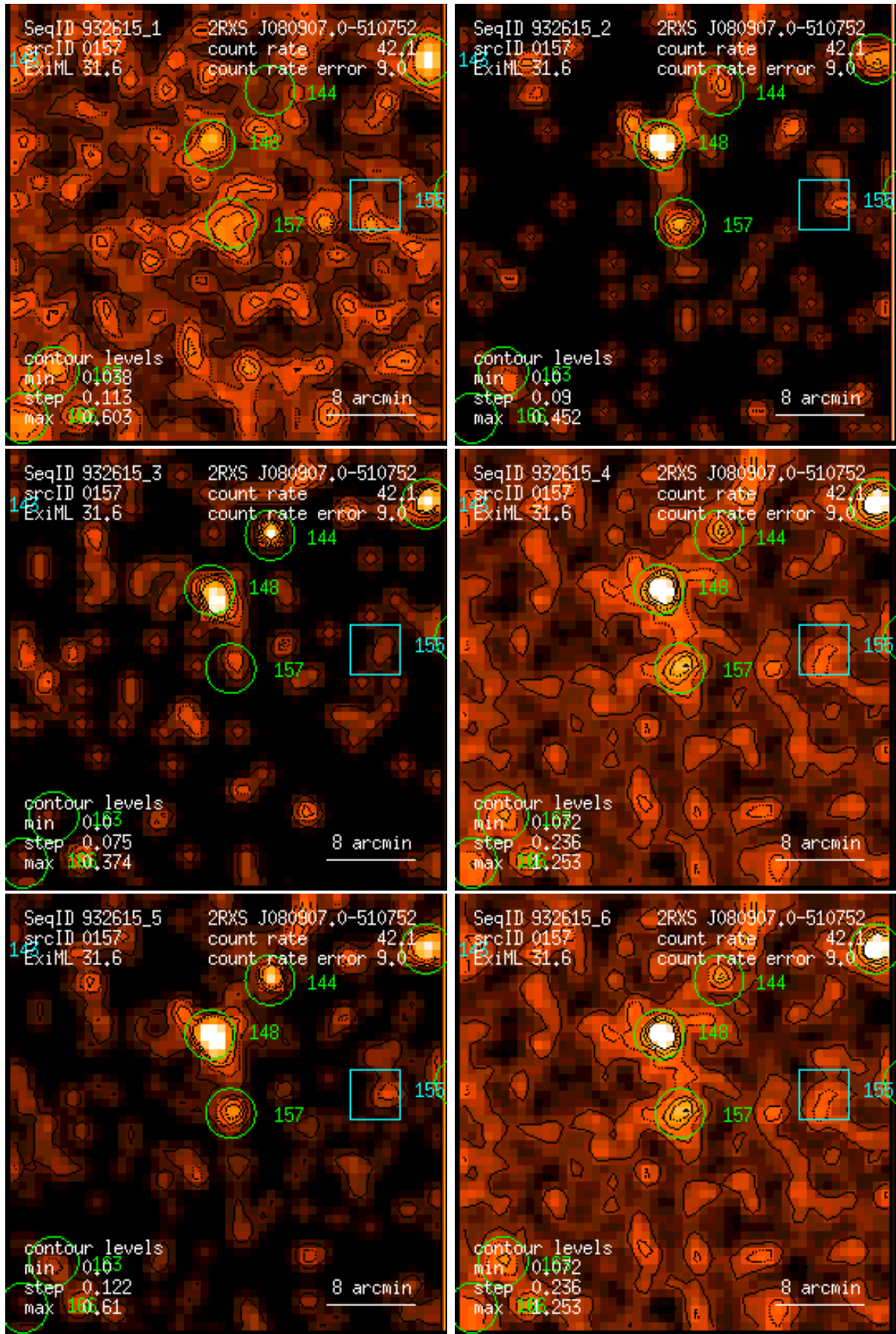
Figure 157: RASS 932615: detection 0157: band rate images, Gaussian filter: (1) PSPC channels 11 – 41, (2) 52 – 90, (3) 91 – 201, (4) 11 – 235, (5) 52 – 201, (6) 11 – 201. Broad band rates in counts/ks. Band rate contour levels in counts/ks/arcmin 2 .
