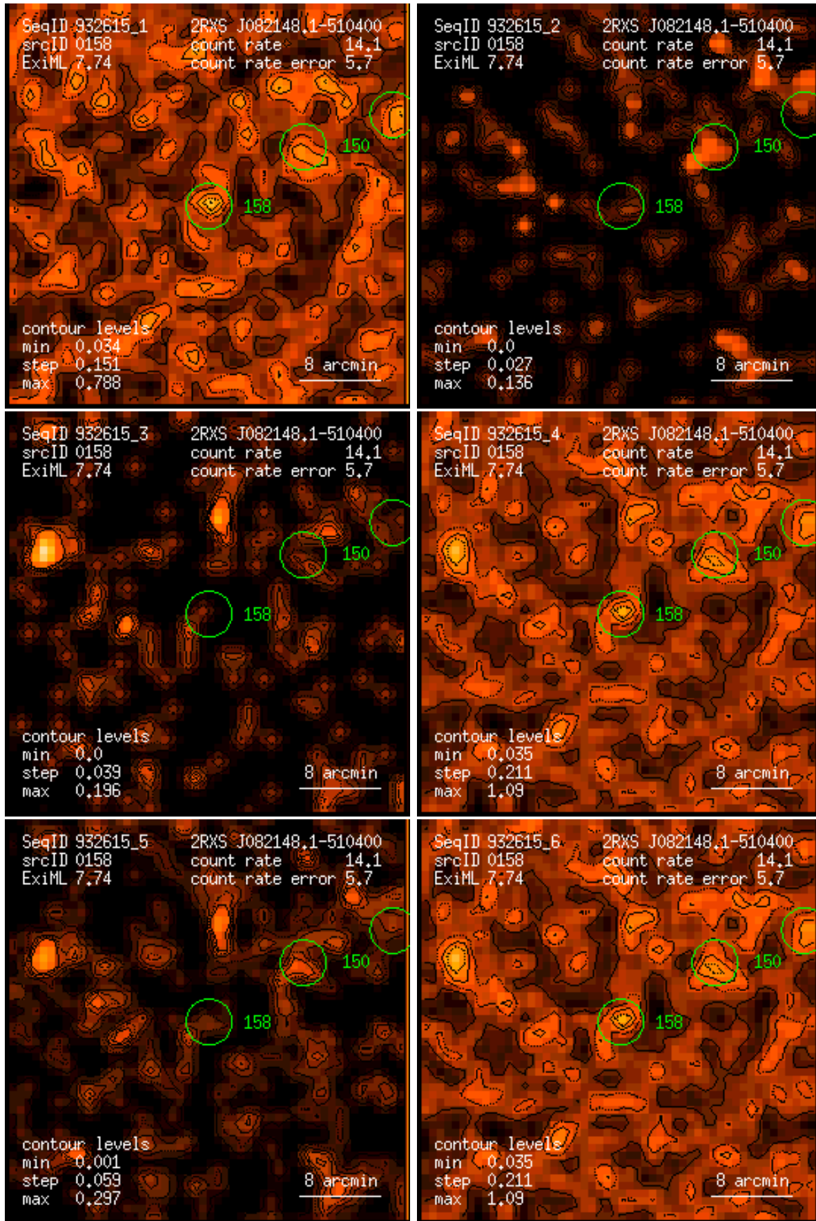
Figure 158: RASS 932615: detection 0158: band rate images, Gaussian filter: (1) PSPC channels 11 – 41, (2) 52 – 90, (3) 91 – 201, (4) 11 – 235, (5) 52 – 201, (6) 11 – 201. Broad band rates in counts/ks. Band rate contour levels in counts/ks/arcmin 2 .
