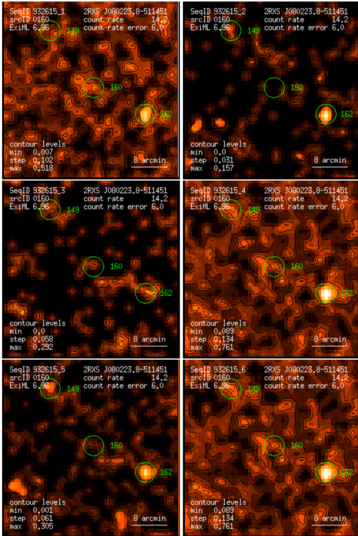
Figure 160: RASS 932615: detection 0160: band rate images, Gaussian filter: (1) PSPC channels 11 – 41, (2) 52 – 90, (3) 91 – 201, (4) 11 – 235, (5) 52 – 201, (6) 11 – 201. Broad band rates in counts/ks. Band rate contour levels in counts/ks/arcmin 2 .
