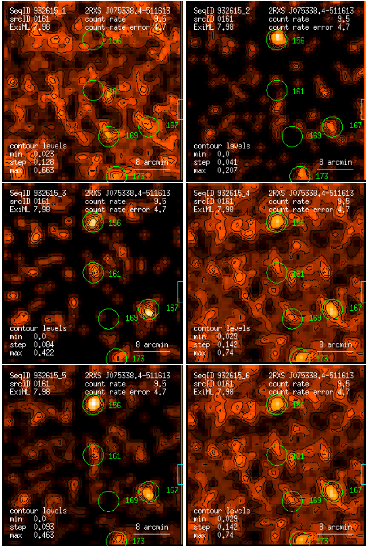
Figure 161: RASS 932615: detection 0161: band rate images, Gaussian filter: (1) PSPC channels 11 – 41, (2) 52 – 90, (3) 91 – 201, (4) 11 – 235, (5) 52 – 201, (6) 11 – 201. Broad band rates in counts/ks. Band rate contour levels in counts/ks/arcmin 2 .
