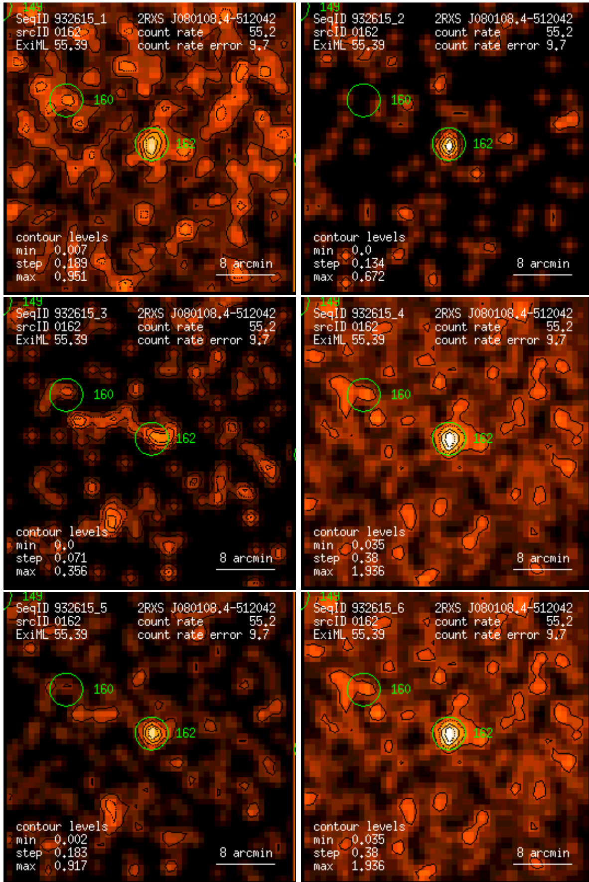
Figure 162: RASS 932615: detection 0162: band rate images, Gaussian filter: (1) PSPC channels 11 – 41, (2) 52 – 90, (3) 91 – 201, (4) 11 – 235, (5) 52 – 201, (6) 11 – 201. Broad band rates in counts/ks. Band rate contour levels in counts/ks/arcmin 2 .
