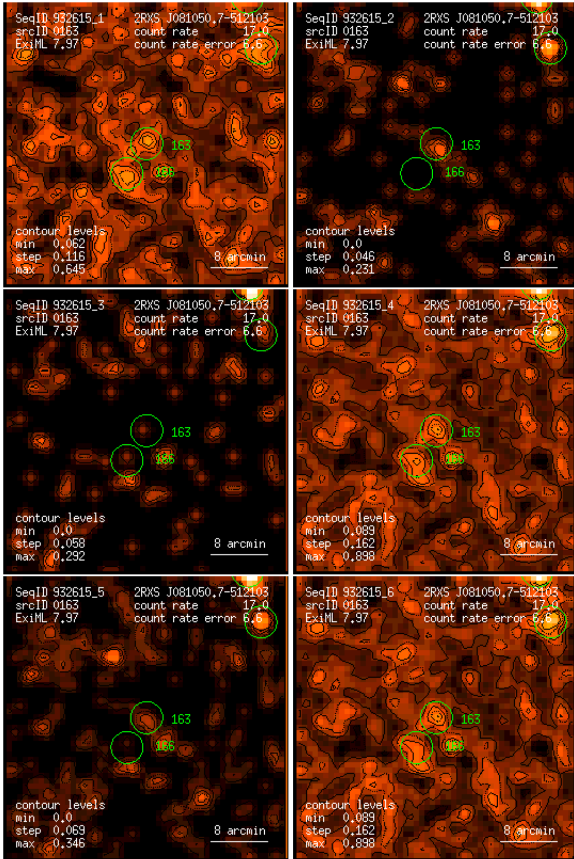
Figure 163: RASS 932615: detection 0163: band rate images, Gaussian filter: (1) PSPC channels 11 – 41, (2) 52 – 90, (3) 91 – 201, (4) 11 – 235, (5) 52 – 201, (6) 11 – 201. Broad band rates in counts/ks. Band rate contour levels in counts/ks/arcmin 2 .
