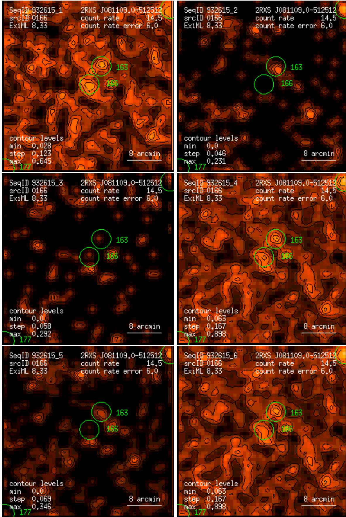
Figure 166: RASS 932615: detection 0166: band rate images, Gaussian filter: (1) PSPC channels 11 – 41, (2) 52 – 90, (3) 91 – 201, (4) 11 – 235, (5) 52 – 201, (6) 11 – 201. Broad band rates in counts/ks. Band rate contour levels in counts/ks/arcmin 2 .
