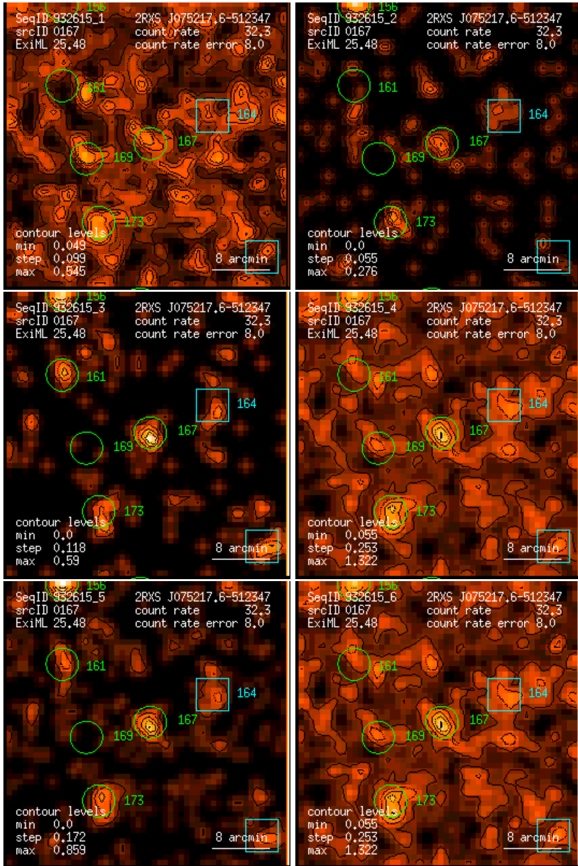
Figure 167: RASS 932615: detection 0167: band rate images, Gaussian filter: (1) PSPC channels 11 – 41, (2) 52 – 90, (3) 91 – 201, (4) 11 – 235, (5) 52 – 201, (6) 11 – 201. Broad band rates in counts/ks. Band rate contour levels in counts/ks/arcmin 2 .
