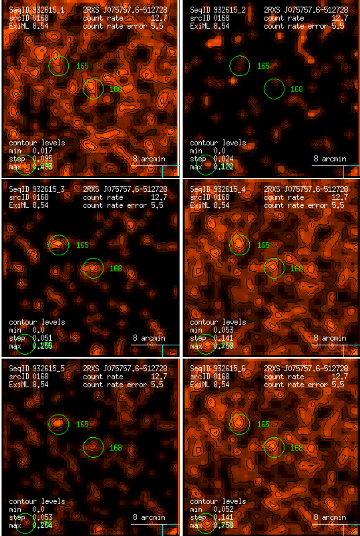
Figure 168: RASS 932615: detection 0168: band rate images, Gaussian filter: (1) PSPC channels 11 – 41, (2) 52 – 90, (3) 91 – 201, (4) 11 – 235, (5) 52 – 201, (6) 11 – 201. Broad band rates in counts/ks. Band rate contour levels in counts/ks/arcmin 2 .
