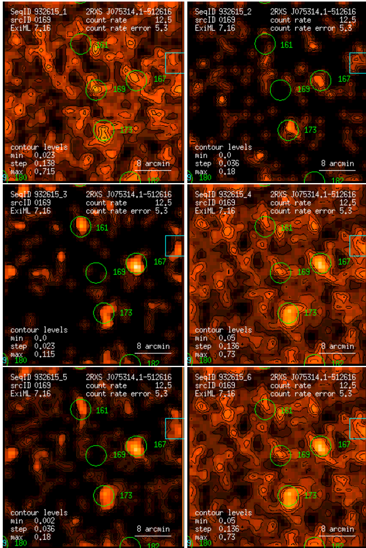
Figure 169: RASS 932615: detection 0169: band rate images, Gaussian filter: (1) PSPC channels 11 – 41, (2) 52 – 90, (3) 91 – 201, (4) 11 – 235, (5) 52 – 201, (6) 11 – 201. Broad band rates in counts/ks. Band rate contour levels in counts/ks/arcmin 2 .
