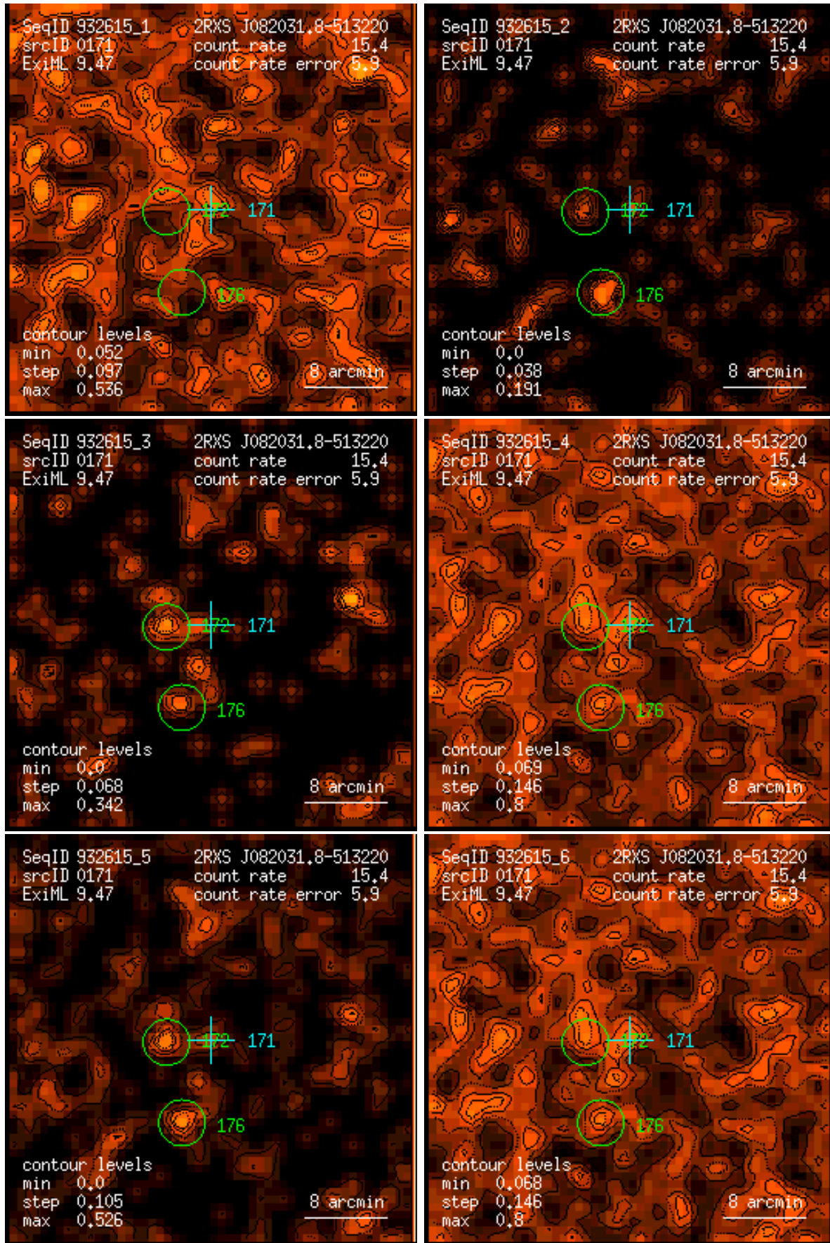
Figure 171: RASS 932615: detection 0171: band rate images, Gaussian filter: (1) PSPC channels 11 – 41, (2) 52 – 90, (3) 91 – 201, (4) 11 – 235, (5) 52 – 201, (6) 11 – 201. Broad band rates in counts/ks. Band rate contour levels in counts/ks/arcmin 2 .
