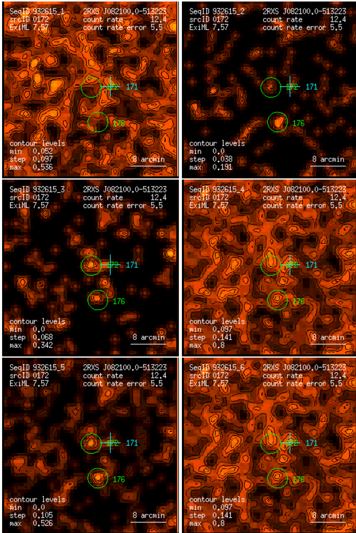
Figure 172: RASS 932615: detection 0172: band rate images, Gaussian filter: (1) PSPC channels 11 – 41, (2) 52 – 90, (3) 91 – 201, (4) 11 – 235, (5) 52 – 201, (6) 11 – 201. Broad band rates in counts/ks. Band rate contour levels in counts/ks/arcmin 2 .
