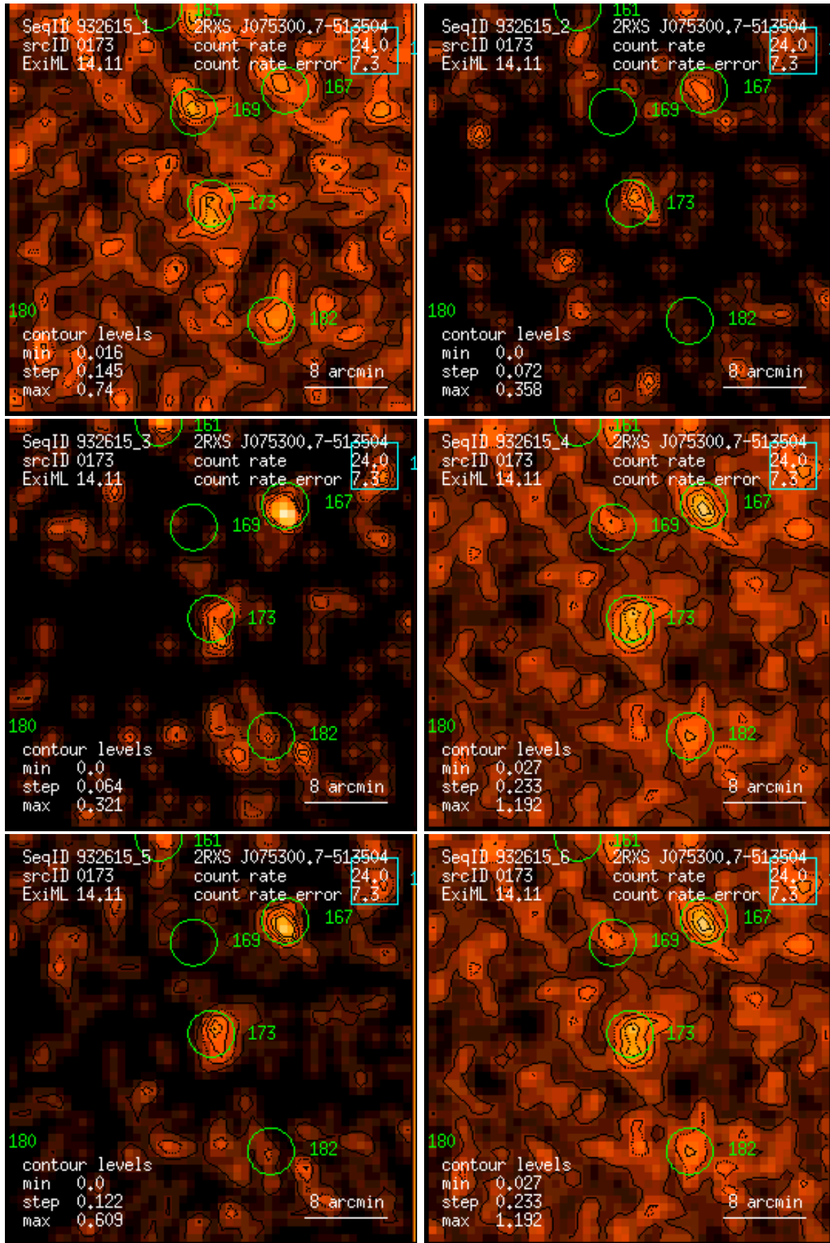
Figure 173: RASS 932615: detection 0173: band rate images, Gaussian filter: (1) PSPC channels 11 – 41, (2) 52 – 90, (3) 91 – 201, (4) 11 – 235, (5) 52 – 201, (6) 11 – 201. Broad band rates in counts/ks. Band rate contour levels in counts/ks/arcmin 2 .
