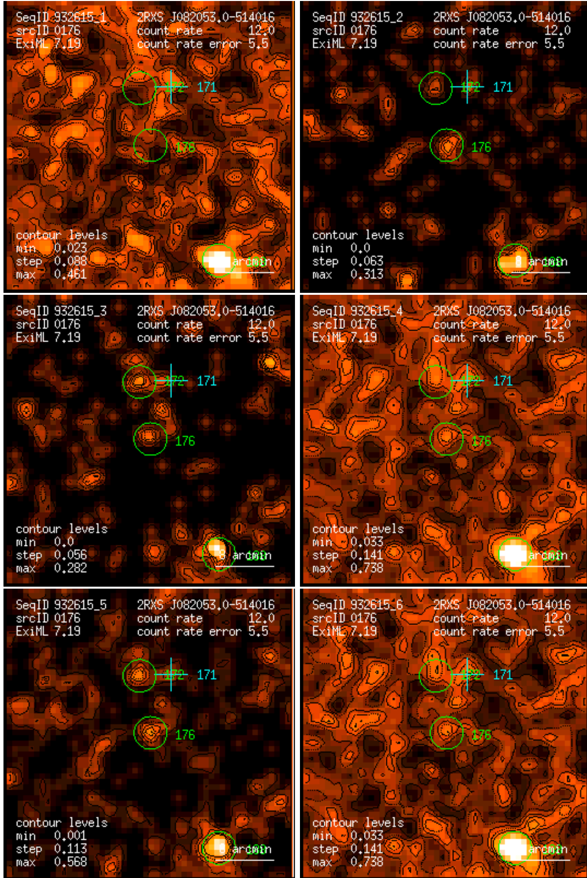
Figure 176: RASS 932615: detection 0176: band rate images, Gaussian filter: (1) PSPC channels 11 – 41, (2) 52 – 90, (3) 91 – 201, (4) 11 – 235, (5) 52 – 201, (6) 11 – 201. Broad band rates in counts/ks. Band rate contour levels in counts/ks/arcmin 2 .
