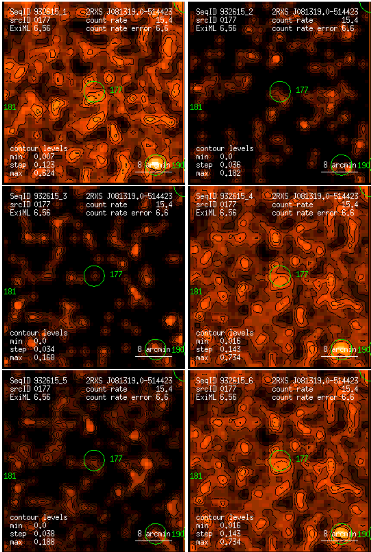
Figure 177: RASS 932615: detection 0177: band rate images, Gaussian filter: (1) PSPC channels 11 – 41, (2) 52 – 90, (3) 91 – 201, (4) 11 – 235, (5) 52 – 201, (6) 11 – 201. Broad band rates in counts/ks. Band rate contour levels in counts/ks/arcmin 2 .
